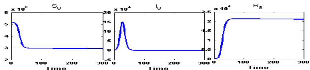
Figure A.39: Susceptible ( S_8 ) class, Infected ( I_8 ) class and Recovered ( R_8 ) class people of Nadia( n_7 ) for fully connected network. After the unlocking, within 28 days, the infected population will reach to its peak value at an amount 1,51,300 persons and down the initial amount of infection in 66 days.
