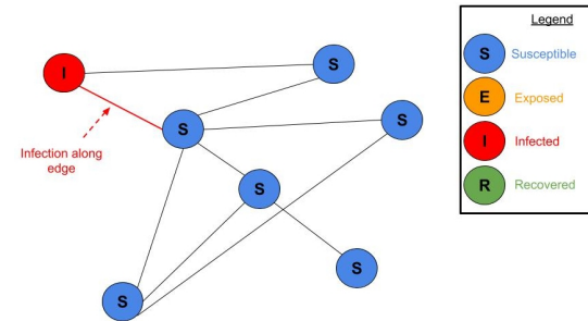
Figure 2: Infected nodes can infect neighboring Susceptible nodes - those who share an edge with them. Full animation at bit.ly/seir-graph-animation .
