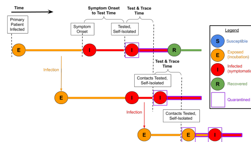
Figure 11: Time intervals in disease and Test & Trace progression.
