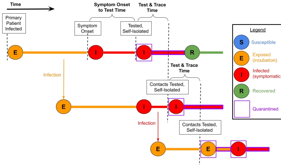
Figure 5: Illustration of the different time intervals in the context of disease progression. Symptom Onset to Test Time is the time from symptom onset to self-isolation and test. Test & Trace Time is the time from when the primary patient is tested and isolated until its contacts are tested and isolated. It is also the time between when the contacts are tested to when their contacts are isolated and tested. Not all contacts are successfully traced, only a certain fraction, Share of Contacts Traced .
