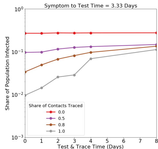
Figure 8: Higher Share of Contacts Traced (color) lines have a steeper slope, meaning for them Test & Trace Time (X axis) has a stronger effect.
