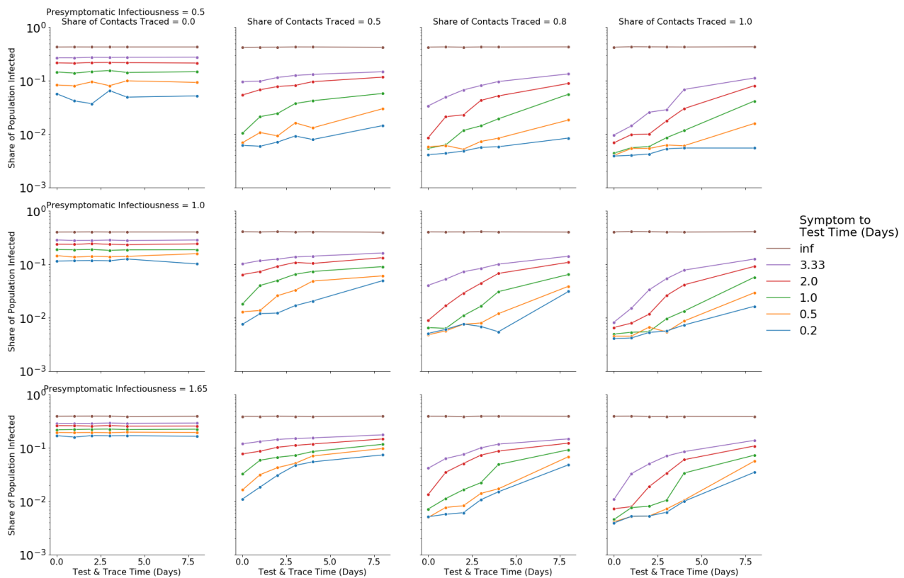
Figure 10: Effects of presymptomatic infectiousness. Each panel shows the effects of Symptom Onset to Test Time (color) and Test & Trace Time (X axis) on Share of Population Infected (Y axis). Columns - Share of Contacts Traced . Rows - presymptomatic relative infectiousness (0.5 - top, 1 - middle, 1.65 - bottom). Presymptomatic infectiousness does not change the relative importance of the main three parameters.
