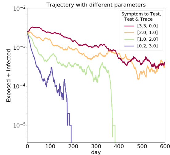
Figure 6: Epidemic trajectories with different time interval parameter values. Plotting over time the (log-scale) share of Exposed and Infected agents in the population. Keeping the sum Symptom Onset to Test Time + Test & Trace Time roughly constant at about 3 days, a shorter Symptom Onset to Test Time facilitates faster containment.
