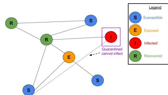
Figure 4: Quarantined node cannot infect others. Susceptible, Exposed, Infected and Recovered nodes shown.
