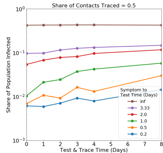
Figure 7: Simulation results varying Symptom Onset to Test Time and of Test & Trace Time . The vertical distance between the different lines is much larger than the vertical distance between the left and right ends of each line. This means changes in Symptom Onset to Test Time are more influential than changes in Test & Trace Time .
