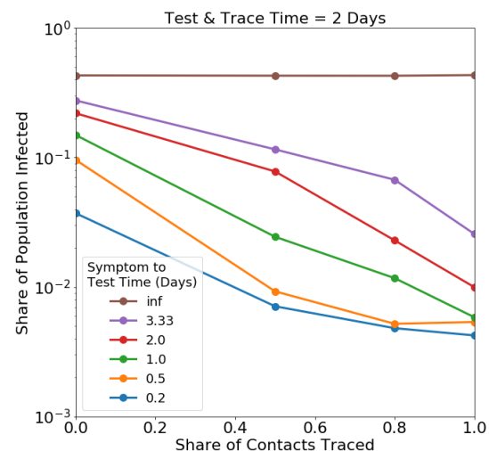
Figure 9: The vertical distance between the colored lines is comparable to the vertical distance between the right side and left side of each line. This means both Share of Contacts Traced and Symptom Onset to Test Time significantly affect the Share of Population Infected.
