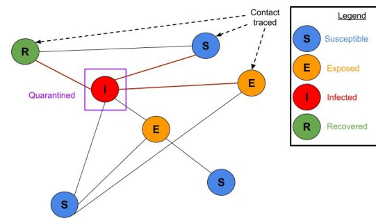
Figure 3: Contact tracing. Share of Contacts Traced of the neighbors of a node which tests positive are traced and themselves self-isolated and tested. In this illustration, 60% of the Infected positive node's contacts were traced (3 out of 5).
