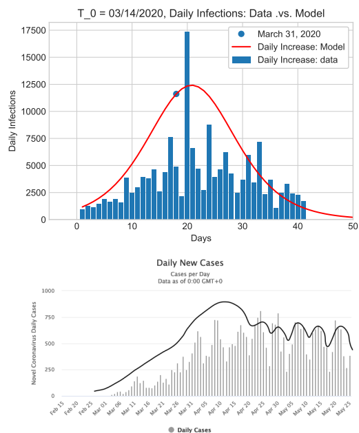
FIG. 4. Number of daily new infections as a function of time for France (top) and Sweden (bottom). The red line in the top plot is the daily infections from our model with constant social distancing d from the week of March 20, 2020. The line in the bottom plot is the envelope of the data (not from our model). When compared to the blue curve in Fig. 3, the shape of data indicates periodically relaxed social distancing during the epidemic and a notable relaxation rate of people wearing face masks in public areas.
