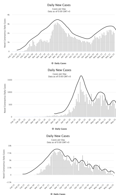
FIG. 5. Number of daily new infections as a function of time for Iran (top), Singapore (middle), and Spain (bottom). The line in each figure is the envelope of the data (not from our model). The epidemic trajectory in Iran suggests that a longer relaxation time is occurring, while the trajectories for Singapore and Spain suggest that most people are wearing masks but the relaxation time is shorter, consistent with more frequent group gatherings.
