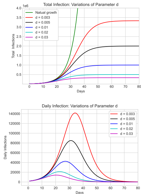
FIG. 1. Total number of infections (top) and daily number of new cases (bottom) versus time as functions of the social distancing parameter d . The red, black, blue, cyan, and purple lines represent increasing social distancing at d = 0.003, 0.005, 0.01, 0.02 , and 0.03 , respectively. The green solid line in the top figure shows the total infections with no intervention, where \gamma = 0.17 .
