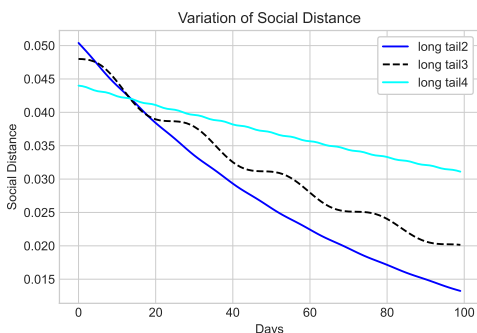
FIG. 2. The effect of social distancing parameter d changing with time. The blue line represents the fast decline of social distancing with a time constant of 11 days (high proportion of people with no face mask). The black dashed line represents slightly less relaxing of social distancing over a longer relaxation period of 24 days. The cyan line denotes a slightly reduced social distancing but with a relaxation period of 7 days.
