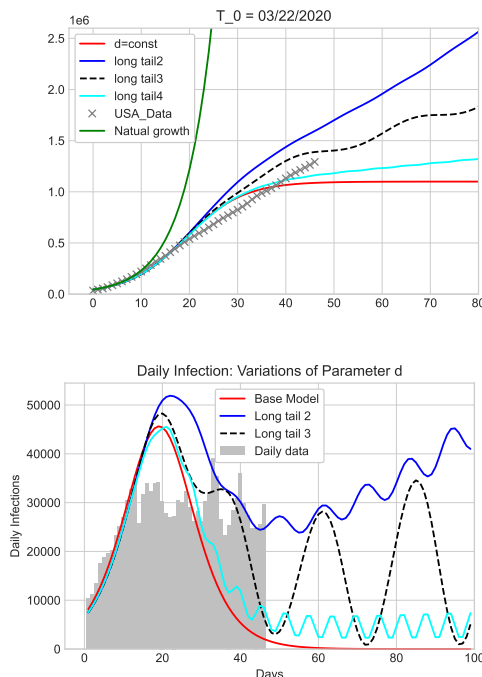
FIG. 3. Total number of infections (top) and number of daily new cases (bottom) changing over time under four social-distancing scenarios. The red line represents the spread trajectory under constant social distancing at the level when restrictions were put in place. The blue line corresponds to social distancing decreasing at a relaxation rate \beta = 1.35\%/day and relaxation time of 11 days. The black dashed line corresponds to 0.9\%/day and 24 days. The cyan line corresponds to 0.35\%/day and T = 7 days. All cases assume a community spread rate of \gamma = 0.17 .
