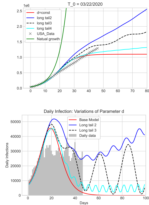
FIG. 3. Total number of infections (top) and number of daily new cases (bottom) changing over time under four social-distancing scenarios. The red line represents the spread trajectory under constant social distancing at the level when restrictions were put in place. The blue line corresponds to social distancing decreasing at a relaxation rate \beta = 1.35\%/day and relaxation time of 11 days. The black dashed line corresponds to 0.9\%/day and 24 days. The cyan line corresponds to 0.35\%/day and T = 7 days. All cases assume a community spread rate of \gamma = 0.17 .
