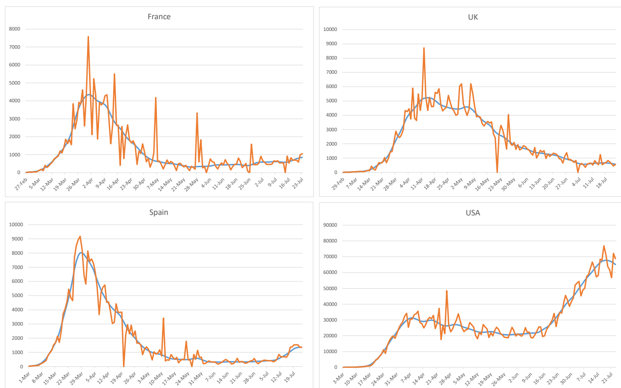
Figure 2: Data of daily infected patients used for comparison with EpiEstim: we show, for the four countries, in orange, the data we used when no filtering was applied and in blue the data after applying a median filter with r_W = 3 and a Gaussian filter with \sigma = 2 .
