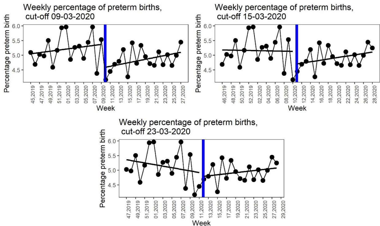
Figure 2: Regression discontinuity in weekly preterm birth incidence surrounding implementation of COVID-19 mitigation measures
