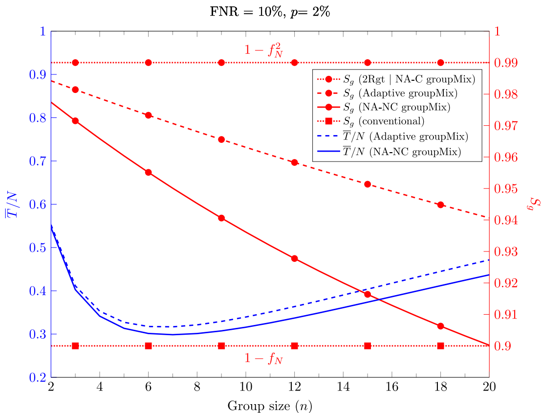
Fig. 2. The average number of tests per sample (left y-axis, blue curves) and group-level sensitivity S_g (right y-axis, red curves) of different methods against the group size.
