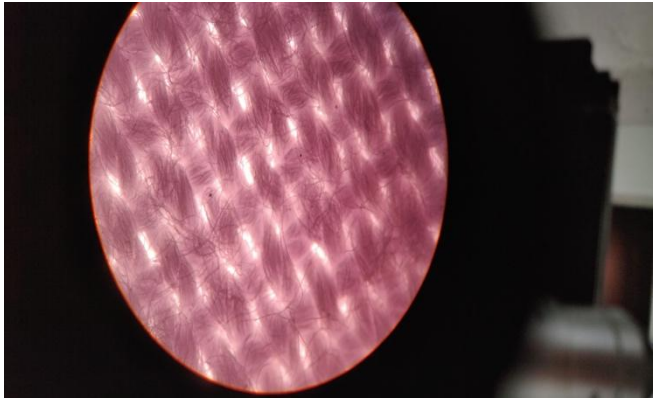
Photo 2: Inner layer of triple layer test mask created by our laboratory (50x)
