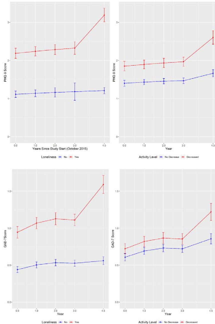
Figure 1 Trajectories of predicted PHQ-9 and GAD-7 scores from zero-inflated negative binomial regression models for loneliness and physical activity
