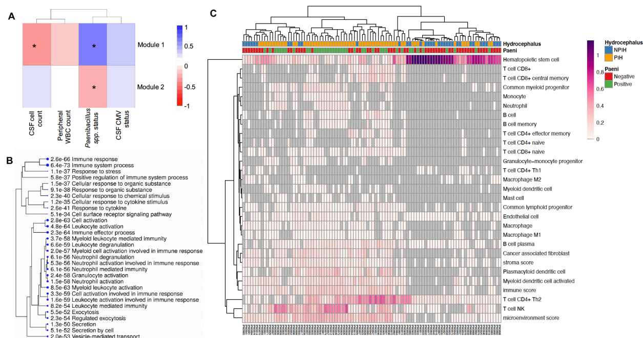
Figure 5: Weighted correlation network analysis (WGCNA) and single cell RNA deconvolution. Panel A demonstrates gene modules within RNA-Seq data for PIH and NPIH cohorts identified by WGCNA. Module 1 negatively correlated with CSF cell count and positively with Paenibacillus spp. status and was enriched for host immune responses, including leukocyte and neutrophil functions (Panel B). Module 2 was negatively correlated with Paenibacillus spp. status, but the associated genes had no specific functional enrichment. Panel C is deconvolution of bulk RNA data into immune cell populations expressed on a scale of 0-1 that calculated for each patient. There was hierarchical clustering of a mixture of NPIH and PIH samples with a hematologic predominance, and PIH-only samples with T-helper and NK cell populations.
