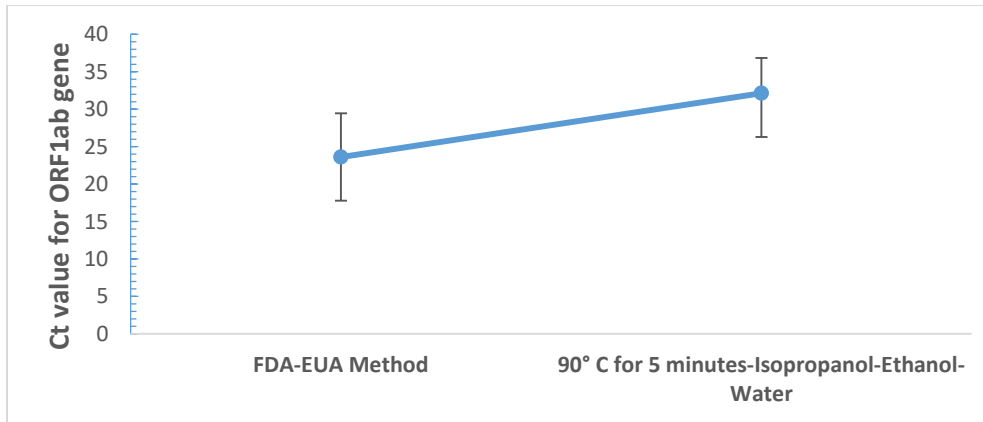
277 Fig 3. The comparison of Ct values for the ORF1ab gene with PerkinElmer Inc. FDA-EUA method vs. alternate method.
