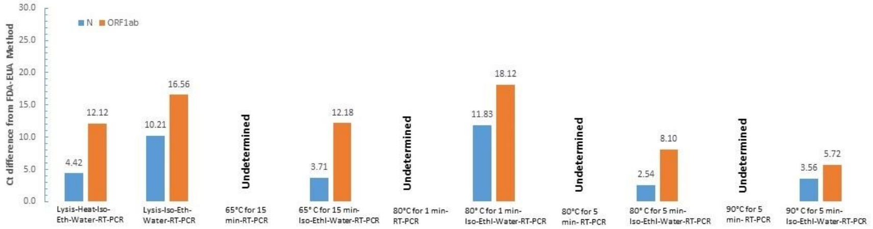
270 Fig 1. Preliminary experiments to optimize alternate RNA extraction method.
