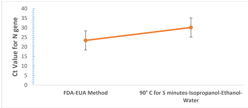
273 Fig 2. The comparison of Ct values for the N gene with PerkinElmer Inc. FDA-EUA method vs. alternate method.
