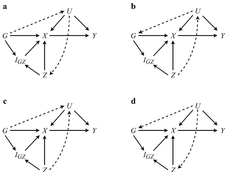
Figure 5: A panel showing a set of 4 DAGs wherein the instrument G and interaction covariate Z are simultaneously associated with one or more confounders U . In this case, DAGs (a), (b), and (d) would likely result in biased causal effect estimates using MR-GxE, in contrast to confounding structure (c).
