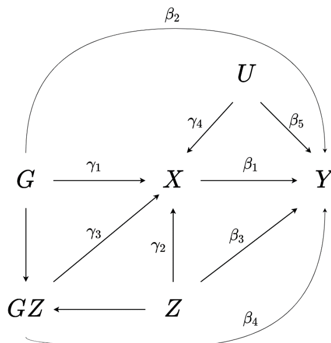
Figure 1: A directed acyclic graph showing the relationship between a genetic instrument G , interaction covariate Z , exposure X , outcome Y , and one or more confounders U . GZ denotes the interaction G \times Z , and G , Z , and U are assumed independent for clarity.
