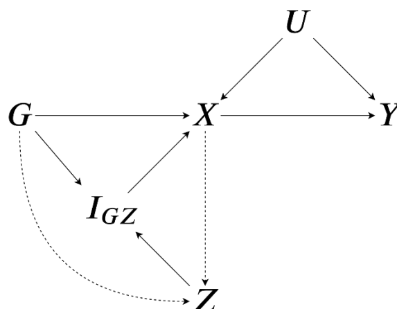
Figure 6: A DAG showing a situation in which conditioning on Z when G and X are simultaneously upstream associated with Z would induce collider bias in a regression of X upon G and Z outlined in equation 5.
