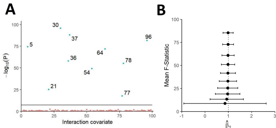
Figure 2: Panel A shows a scatter plot of -\log_{10}(p\text{-value}) for the first-stage F-statistic across the set of 100 potential interaction covariates for a single simulated data set. Panel B shows a forest plot of mean causal effect estimates and confidence intervals under varying mean interaction strength. A solid horizontal line is included representing the Bonferroni correction threshold for statistical significance in panel A, while the dotted vertical line in panel B represents the true causal effect \beta_1 = 1 .
