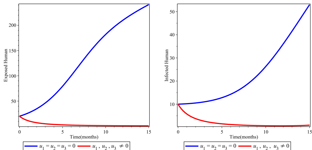
Figure 5: Simulations of the model with all control strategies.
