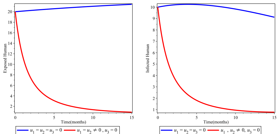
Figure 2: Simulations of the COVID 19 model with preventive measure & supporting infectives with medication .
