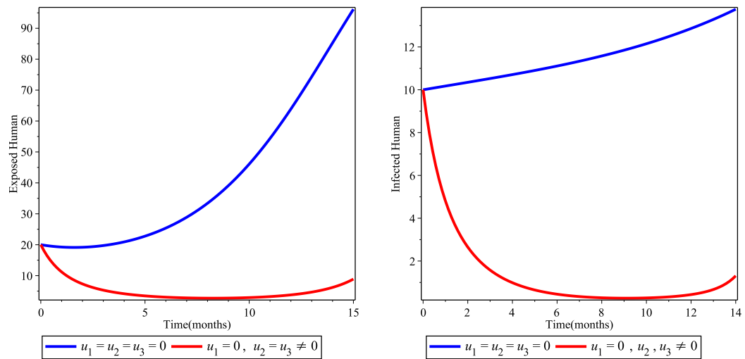
Figure 4: Simulations of the COVID 19 model with Supporting infectives with medication & Media campaign .
