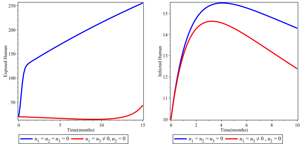
Figure 3: Simulations of the COVID 19 model with Social distancing with personal hygiene & Media campaign .
