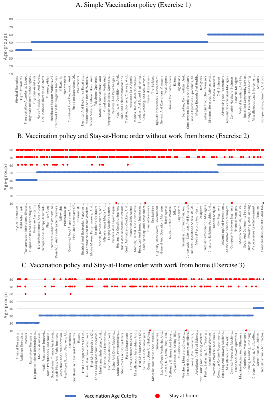
Figure A.2: Age cutoffs for vaccinations and age groups staying at home when vaccine effectiveness is 0.7. Occupations on the x-axis are ordered based on their infection risk. (A) The optimal vaccination policy showing the youngest age for each occupation that is eligible to receive the vaccine. (B) The optimal vaccination policy showing the youngest age for each occupation that is eligible to receive the vaccine, together with the occupation-age groups that are mandated to stay at home. (C) The optimal vaccination policy showing the youngest age for each occupation which cannot be done from home that is eligible to receive the vaccine, together with the occupation-age groups that are mandated to stay at home. Occupations that can be done from home do not receive a vaccine.
