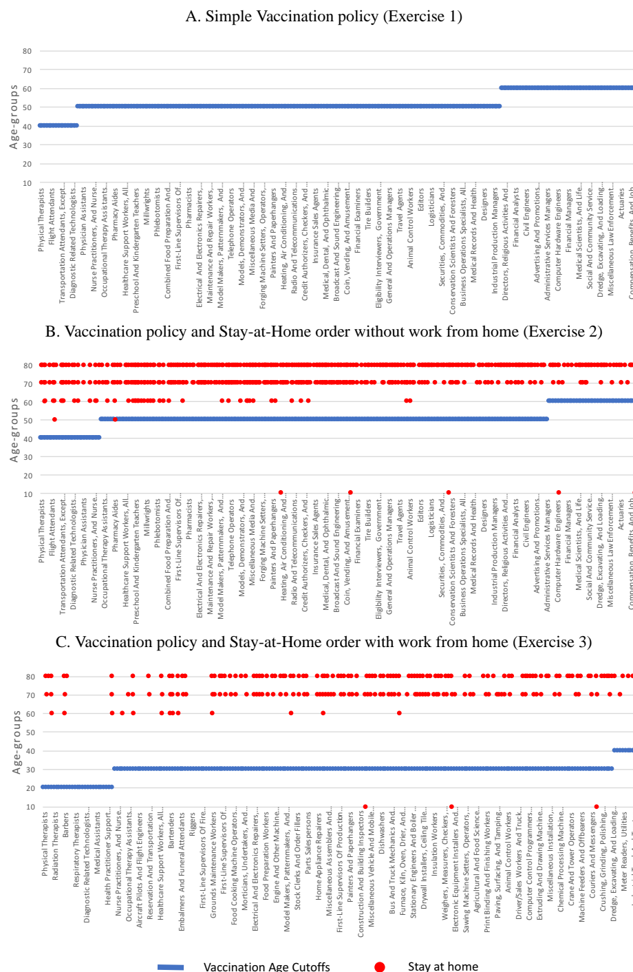
Figure 1: Age cutoffs for vaccinations and age groups staying at home. Occupations on the x-axis are ordered based on their infection risk. (A) The optimal vaccination policy showing the youngest age for each occupation that is eligible to receive the vaccine. (B) The optimal vaccination policy showing the youngest age for each occupation that is eligible to receive the vaccine, together with the occupation-age groups that are mandated to stay at home. (C) The optimal vaccination policy showing the youngest age for each occupation which cannot be done from home that is eligible to receive the vaccine, together with the occupation-age groups that are mandated to stay at home. Occupations that can be done from home do not receive a vaccine.
