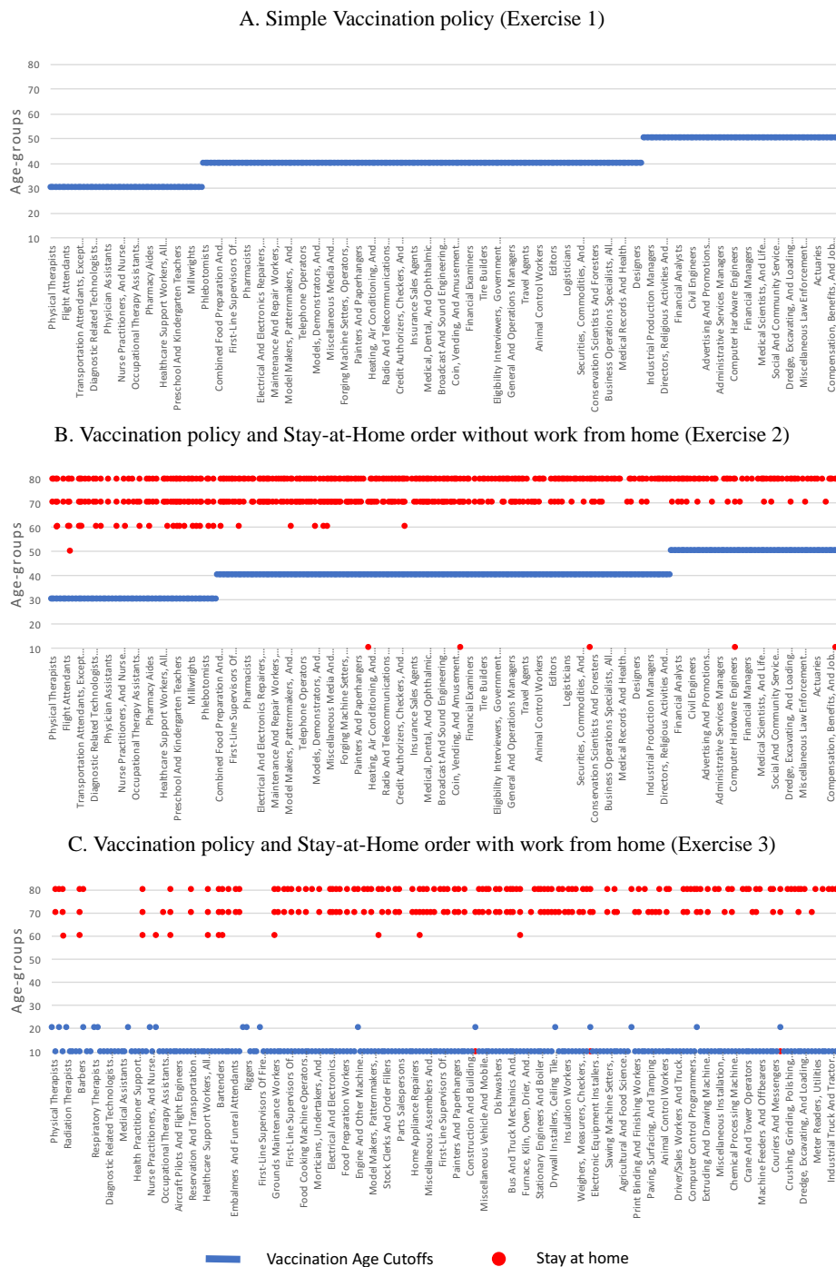
Figure A.4: Age cutoffs for vaccinations and age groups staying at home, when the supply of vaccines is 100mil doses. Occupations on the x-axis are ordered based on their infection risk. (A) The optimal vaccination policy showing the youngest age for each occupation that is eligible to receive the vaccine. (B) The optimal vaccination policy showing the youngest age for each occupation that is eligible to receive the vaccine, together with the occupation-age groups that are mandated to stay at home. (C) The optimal vaccination policy showing the youngest age for each occupation which cannot be done from home that is eligible to receive the vaccine, together with the occupation-age groups that are mandated to stay at home. Occupations that can be done from home do not receive a vaccine. Note: While, in exercise 3, the vaccination cutoffs may appear to be non-monotonic in occupations' risks, that is only because some occupations have no teenage workers.
