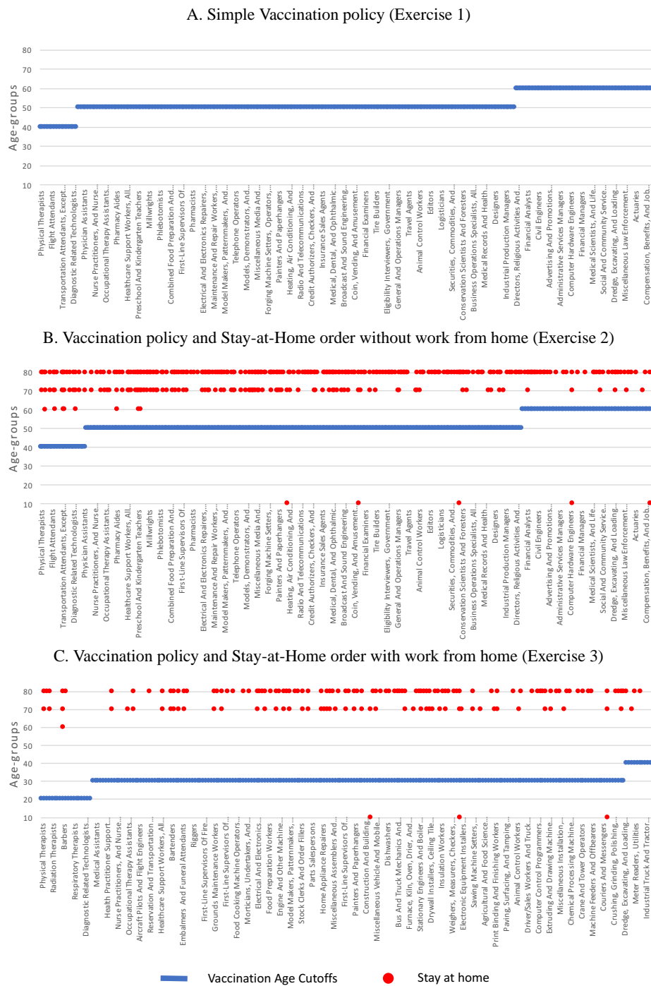
Figure A.6: Age cutoffs for vaccinations and age groups staying at home based on South-Korean infection fatality rates from Table A.2. Occupations on the x-axis are ordered based on their infection risk. (A) The optimal vaccination policy showing the youngest age for each occupation that is eligible to receive the vaccine. (B) The optimal vaccination policy showing the youngest age for each occupation that is eligible to receive the vaccine, together with the occupation-age groups that are mandated to stay at home. (C) The optimal vaccination policy showing the youngest age for each occupation which cannot be done from home that is eligible to receive the vaccine, together with the occupation-age groups that are mandated to stay at home. Occupations that can be done from home do not receive a vaccine.
