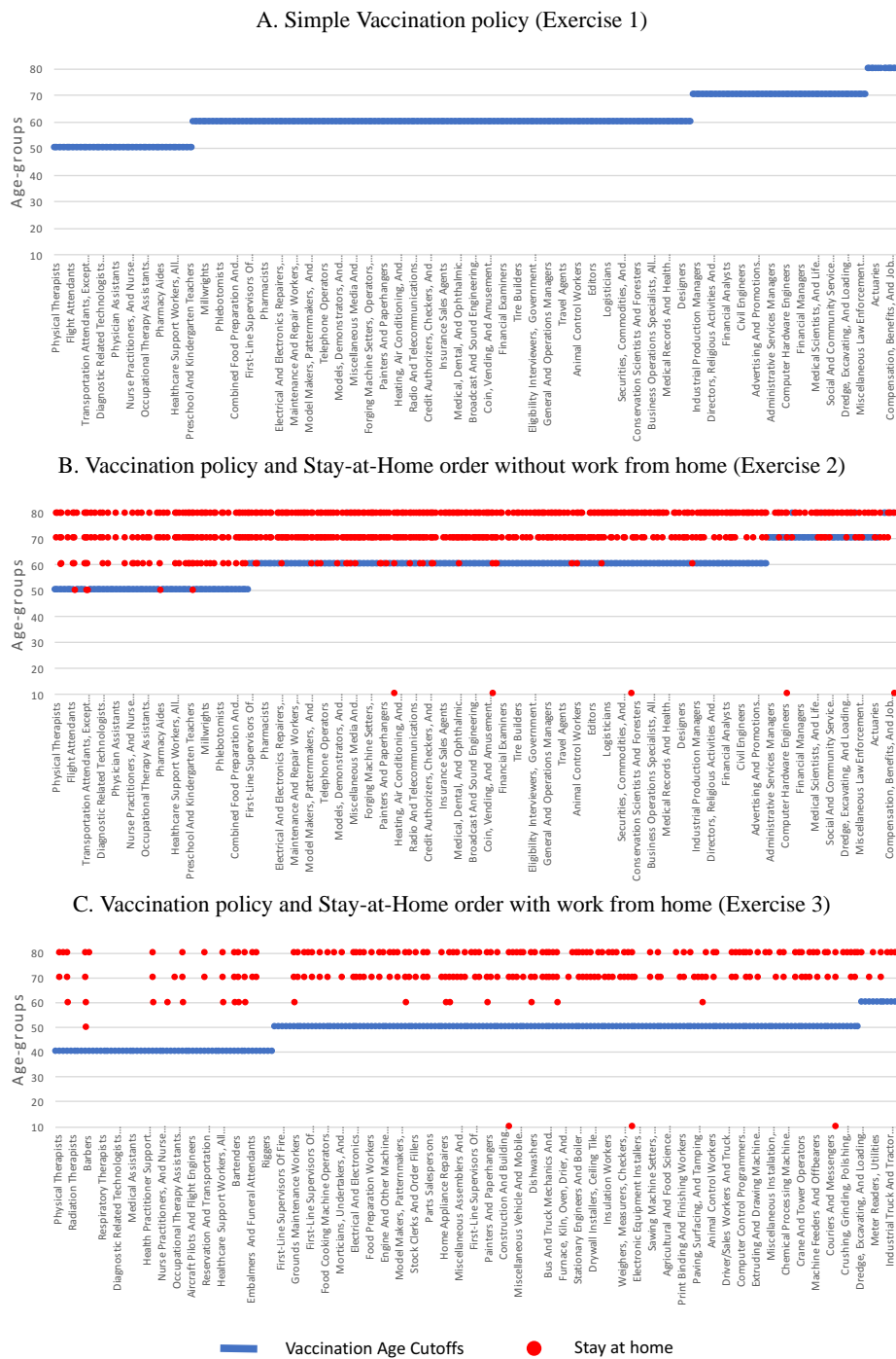
Figure A.3: Age cutoffs for vaccinations and age groups staying at home, when the supply of vaccines is 30mil doses. Occupations on the x-axis are ordered based on their infection risk. (A) The optimal vaccination policy showing the youngest age for each occupation that is eligible to receive the vaccine. (B) The optimal vaccination policy showing the youngest age for each occupation that is eligible to receive the vaccine, together with the occupation-age groups that are mandated to stay at home. (C) The optimal vaccination policy showing the youngest age for each occupation which cannot be done from home that is eligible to receive the vaccine, together with the occupation-age groups that are mandated to stay at home. Occupations that can be done from home do not receive a vaccine.
