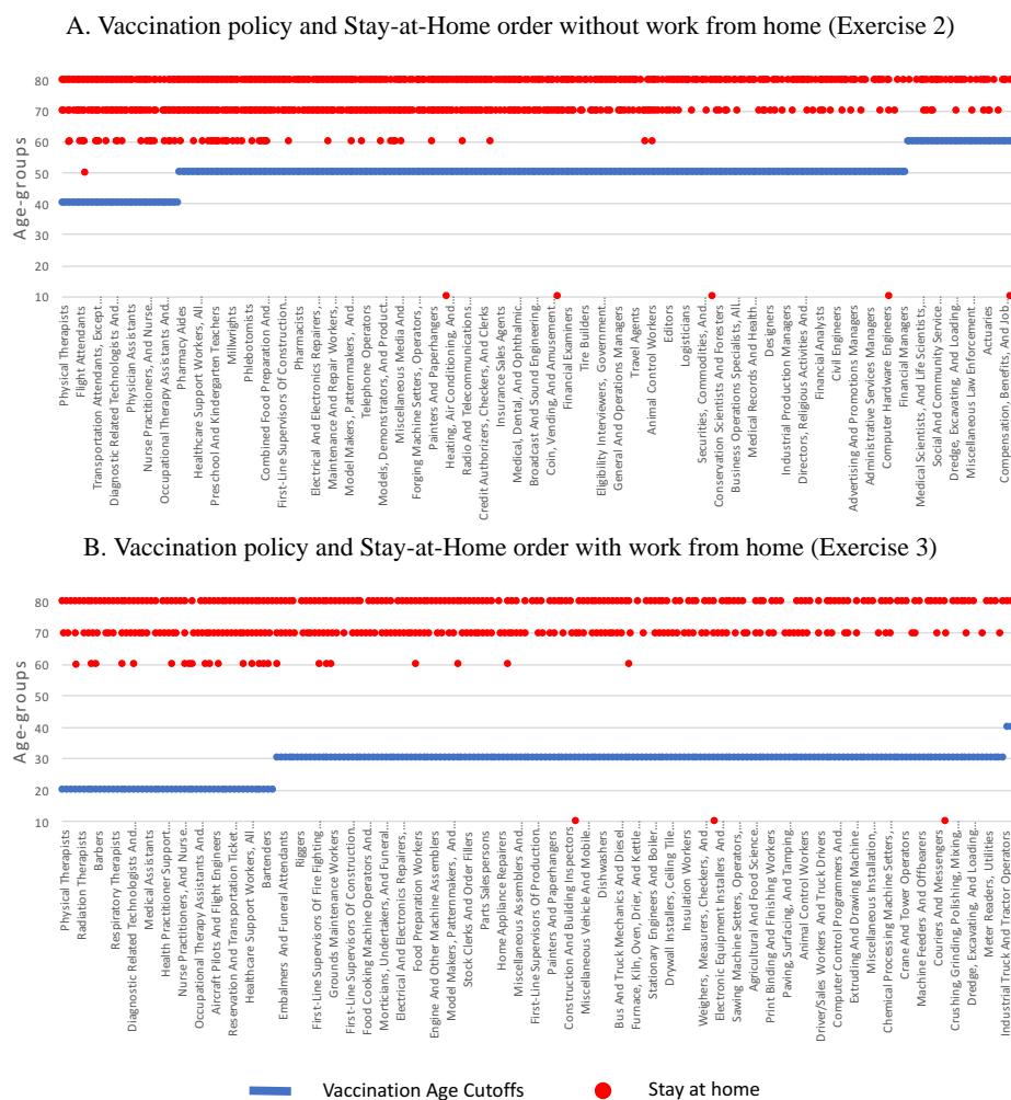
Figure A.1: Age cutoffs for vaccinations and age groups staying at home when no occupations are designated to be essential. Occupations on the x-axis are ordered based on their infection risk. (A) The optimal vaccination policy showing the youngest age for each occupation that is eligible to receive the vaccine, together with the occupation-age groups that are mandated to stay at home. (B) The optimal vaccination policy showing the youngest age for each occupation, which cannot be done from home that is eligible to receive the vaccine, together with the occupation-age groups that are mandated to stay at home. Occupations that can be done from home do not receive a vaccine.
