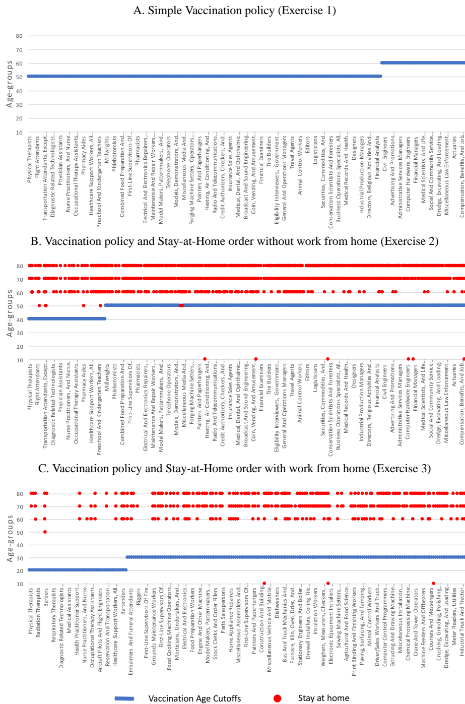
Figure A.5: Age cutoffs for vaccinations and age groups staying at home (probit estimation including all ages mortality risk, \alpha=-1.152288 and \beta=0.0037667 ). Occupations on the x-axis are ordered based on their infection risk. (A) The optimal vaccination policy showing the youngest age for each occupation that is eligible to receive the vaccine. (B) The optimal vaccination policy showing the youngest age for each occupation that is eligible to receive the vaccine, together with the occupation-age groups that are mandated to stay at home. (C) The optimal vaccination policy showing the youngest age for each occupation which cannot be done from home that is eligible to receive the vaccine, together with the occupation-age groups that are mandated to stay at home. Occupations that can be done from home do not receive a vaccine.
