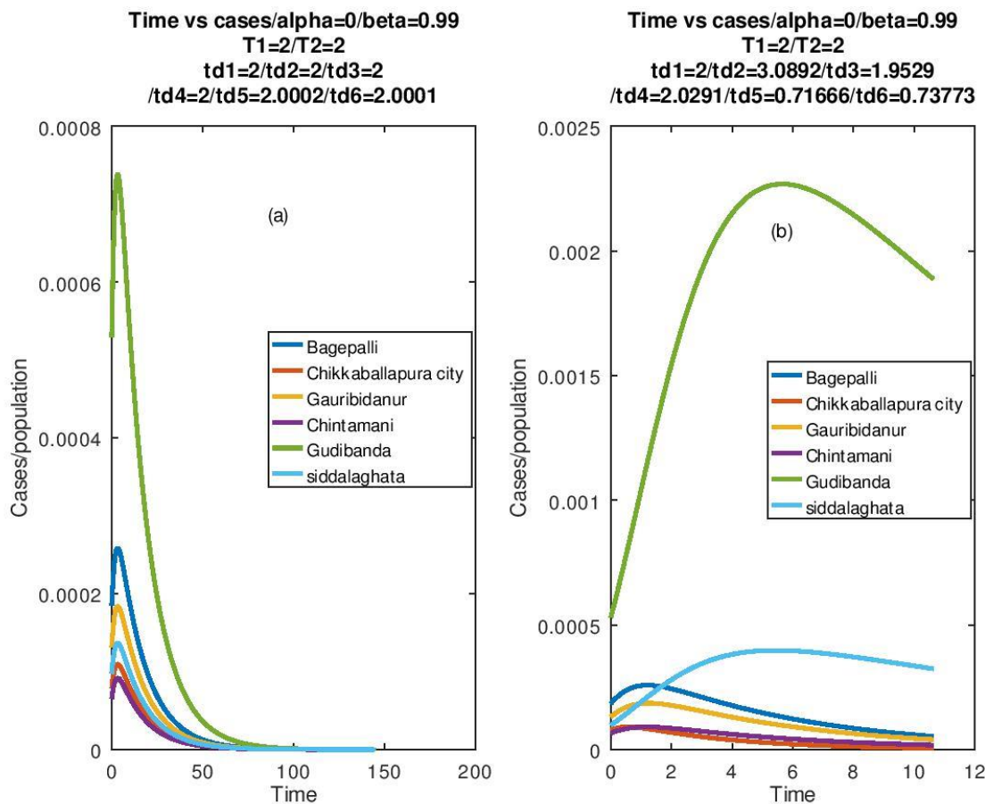
Figure 9. Growth curves for cases in Table 2. In subplot (a), the F 's were adjusted to give the initial doubling time for all cases to be 2 days keeping \alpha(t) = 0 and \beta(t) rises from \beta(0) = 0 to \beta(\infty) = 0.99 . It is seen that all of them decay. In subplot (b), F is kept fixed for all cases and we find that their growth curves differ, but qualitatively they decay after an initial growth. The t_d 's designate the doubling times for the different towns.
