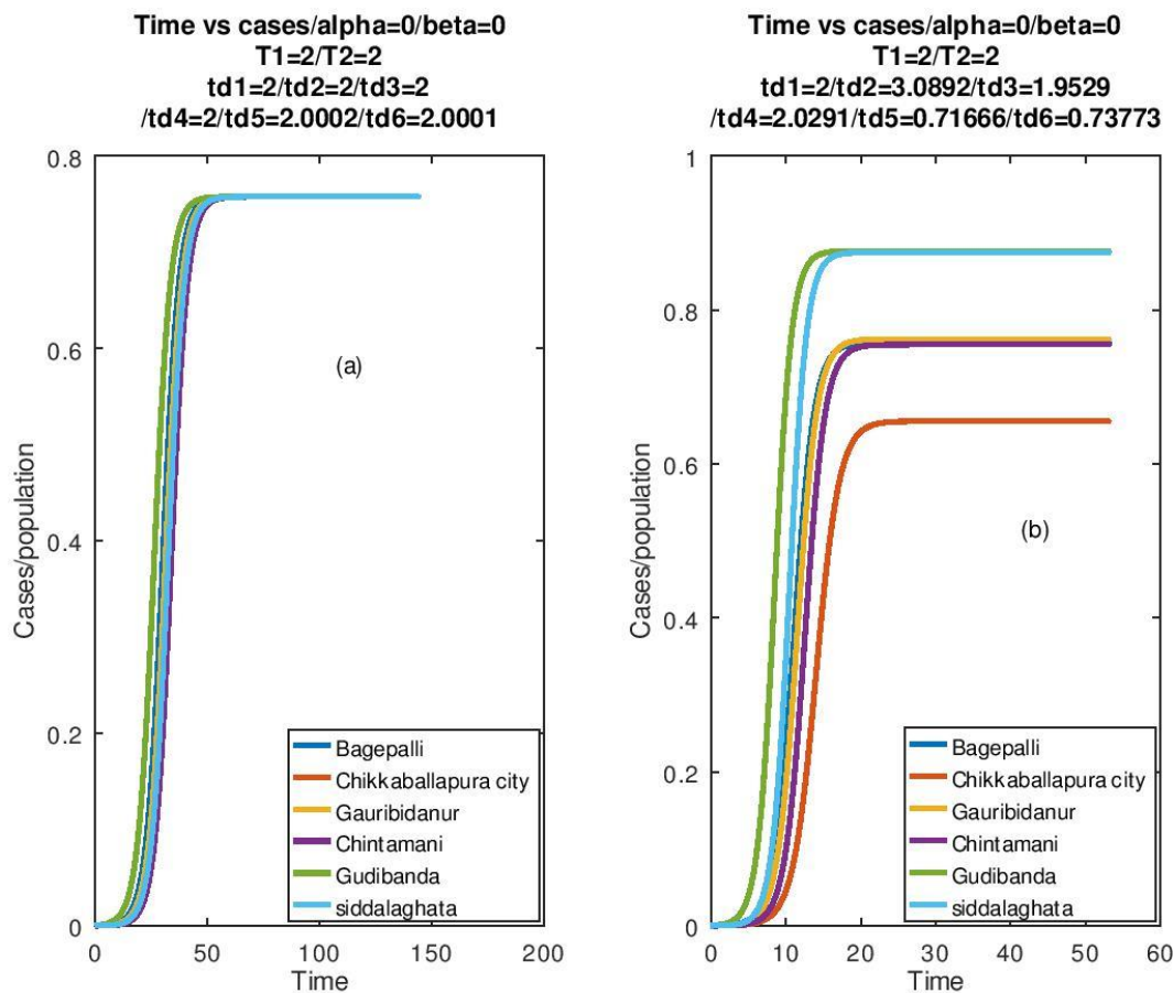
Figure 7. Growth curves for cases in Table 2. In subplot (a) the F 's were adjusted to give the initial doubling time for all cases to be 2 days keeping \alpha(t) = 0 = \beta(t) . It is seen that all of them reach the same [x(t)/N] as t \rightarrow \infty . In subplot (b) F is kept fixed for all cases and we find that they saturate at different [x(t)/N] . The t_d 's designate the doubling times for the different towns.
