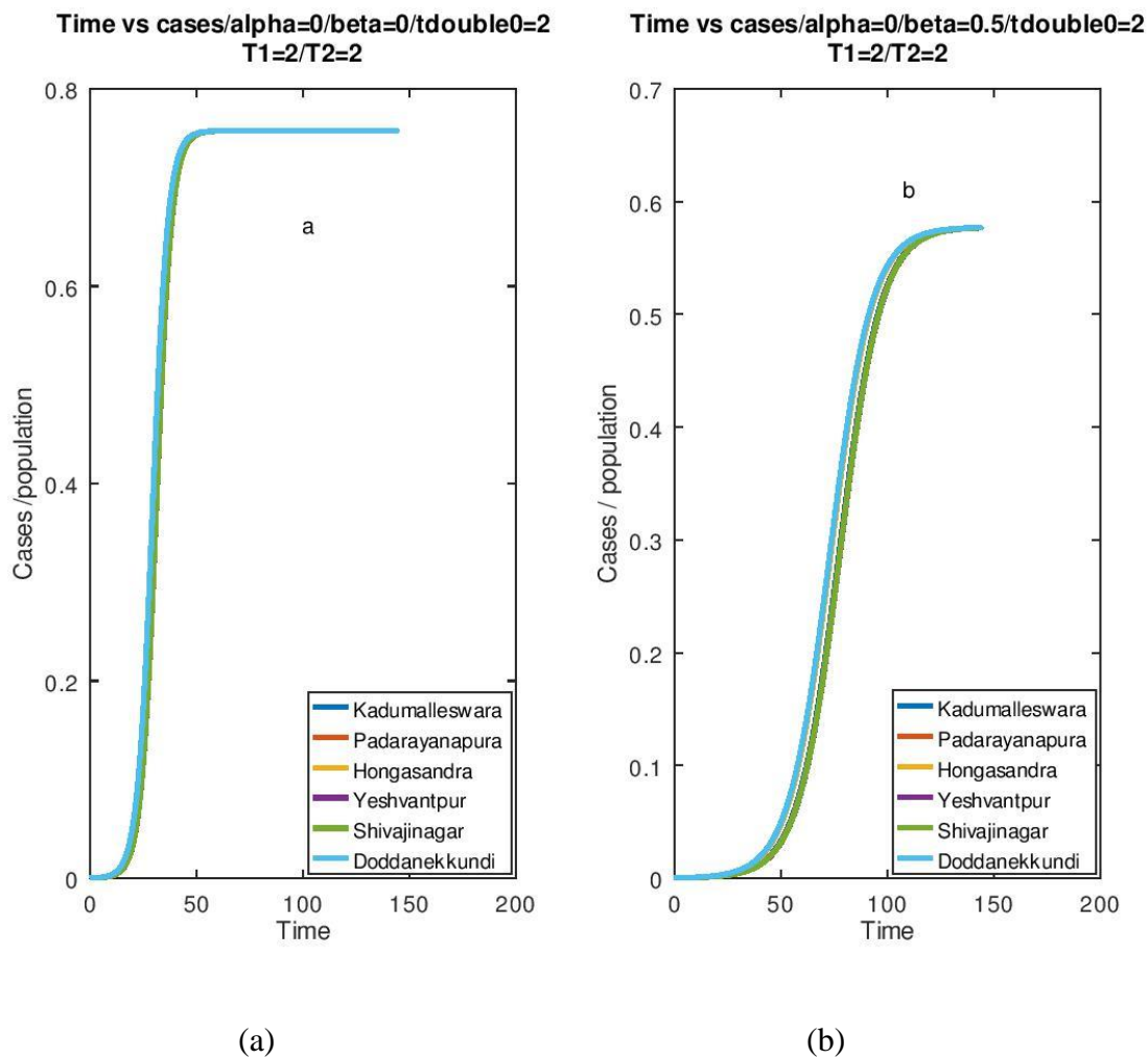
Figure 2: In both graphs T_1=T_2=doubletime0= t_{double} = 2 days. In the graph (a) \alpha(t)=0 and \beta(t) = 0 . In graph (b) \alpha(t)=0 and \beta(\infty)=0.5 . The different curves in both plots are overlapping.
