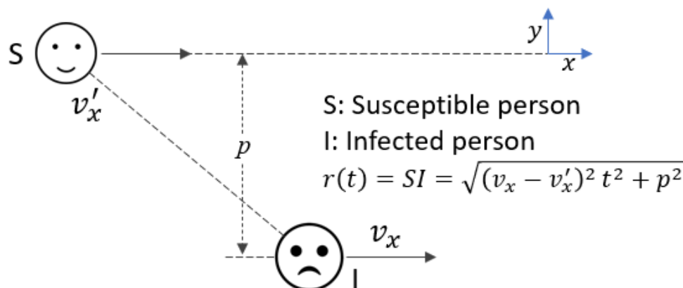
Figure1. Geometry of encounter between the infected person (I) and the susceptible person (S), with their velocities being v_x and v'_x , respectively in the x-direction, with p being the impact parameter.
