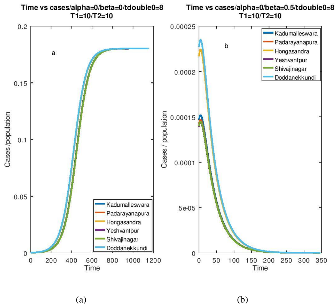
Figure 5: In both graphs T_1=T_2=10 days and \text{doubletime0}=t_{\text{double}}=8 days. In the graph (a) \alpha(t)=0 and \beta(t)=0 . In graph (b) \alpha=0 and \beta=0.5 . The different curves in both plots show similar trend. In plot (a), cases reach saturation, whereas in plot (b), decrease in cases over time is seen.
