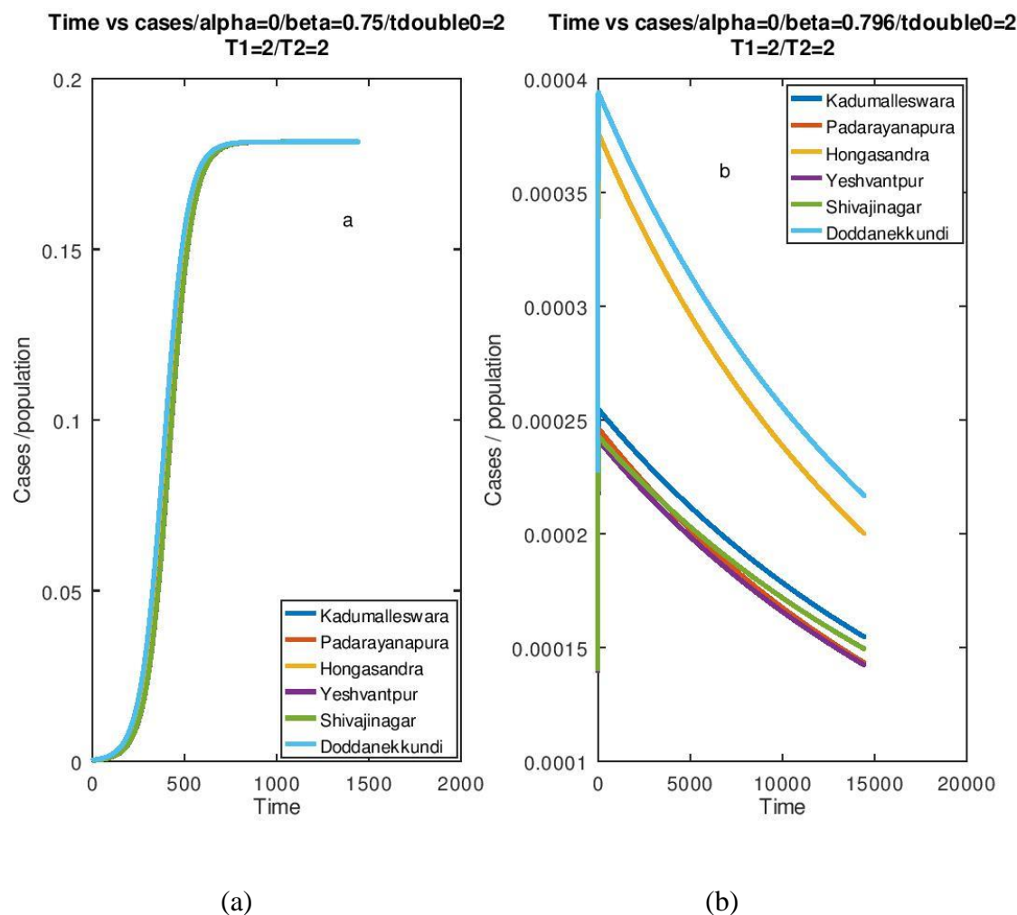
Figure 3: In both graphs T_1=T_2= \text{doubletime0} = t_{\text{double}} = 2 \text{ days} . In the graph (a) \alpha(t)=0 and \beta(\infty)=0.75 . In graph (b) \alpha(t)=0 and \beta(\infty)=0.796 . The different curves in both plots show similar trend. In plot (a), the cases reach saturation but in plot (b), we find a decrease in the number of cases, although over a very long period of time.
