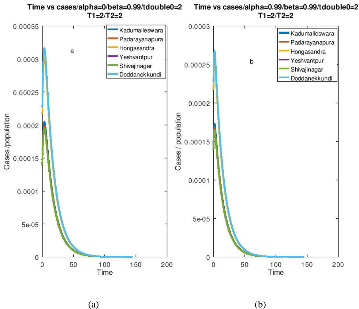
Figure 4: In both graphs T_1=T_2= \text{doubletime0}= t_{\text{double}} = 2\text{days} . In the graph (a) \alpha(t)=0 and \beta(t)=0.99 . In graph (b) \alpha(t)=0.99 and \beta(t)=0.99 . The different curves in both plots show similar trend. Both plots show the cases going to zero in about 100 – 150 days.
