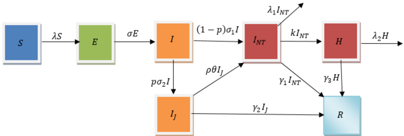
Figure 1. The systematic diagram of the COVID-19 model
