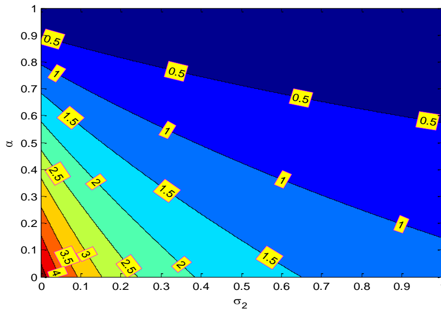
Figure 3. Contour plot for the basic reproduction number, ( R_0 ), of the COVID-19 model as a function of mass testing ( \sigma_2 ) and intervention measures, ( \alpha ).
