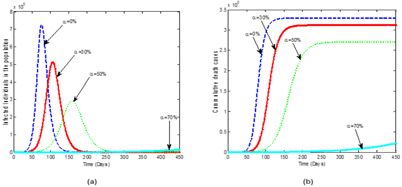
Figure 5. Simulation solution of the COVID-19 model of equation (3) when the compliance of intervention measures, \alpha , is increasing with testing rate, \sigma_2 = 0.061 for (a) the infected individuals in the population and (b) cumulative death cases.
