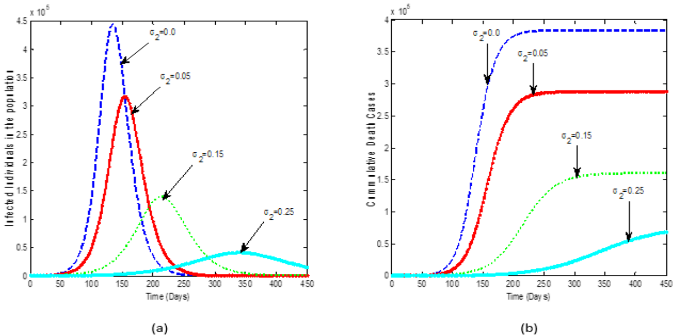
Figure 4. Simulation solution of the COVID-19 model of equation (3) when testing rate, \sigma_2 , is increasing in the presence of compliance of intervention measures, \alpha = 50\% for (a) the infected individuals in the population and (b) cumulative death cases.
