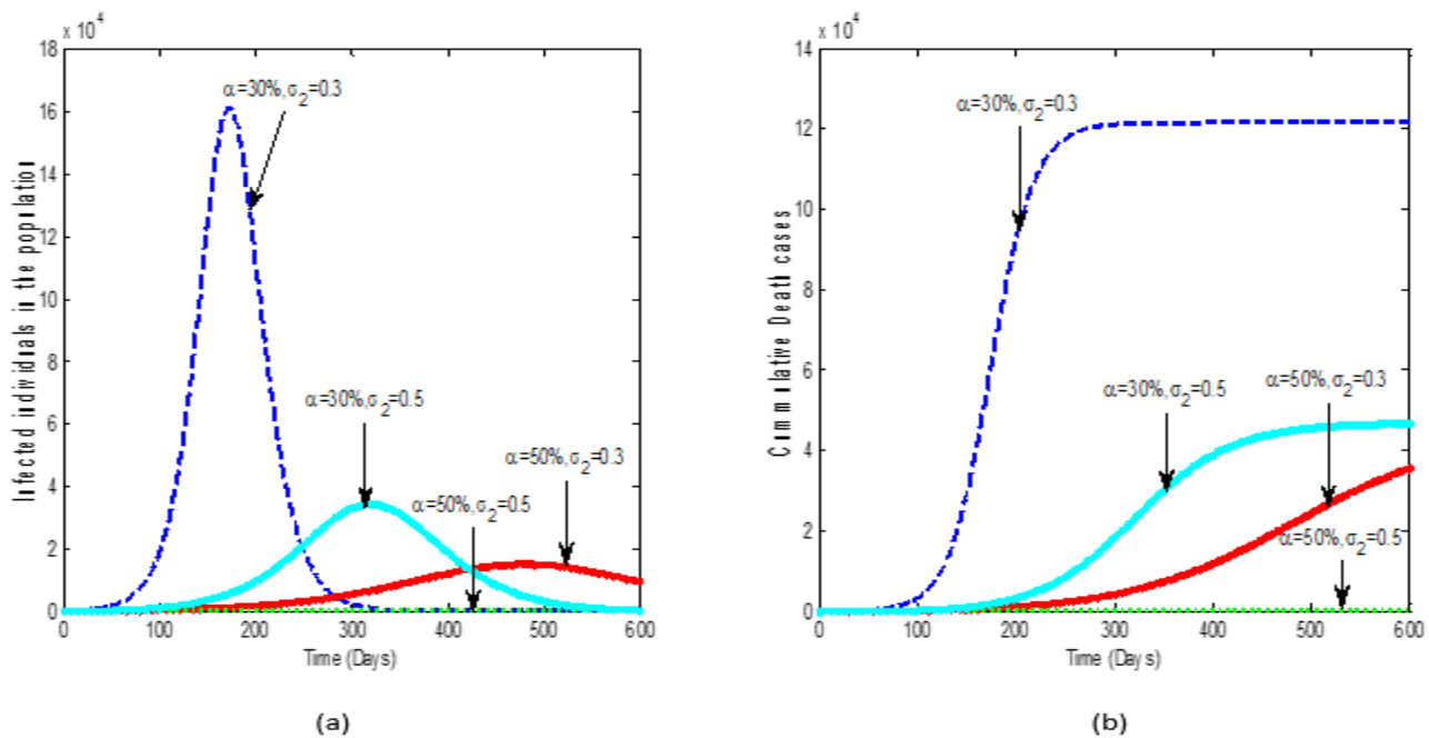
Figure 6. Simulation solution of the COVID-19 model of equation (3) when both the testing rate, \sigma_2 , and compliance of intervention measures, \alpha , are increasing for (a) the infected individuals in the population and (b) cumulative death cases.
