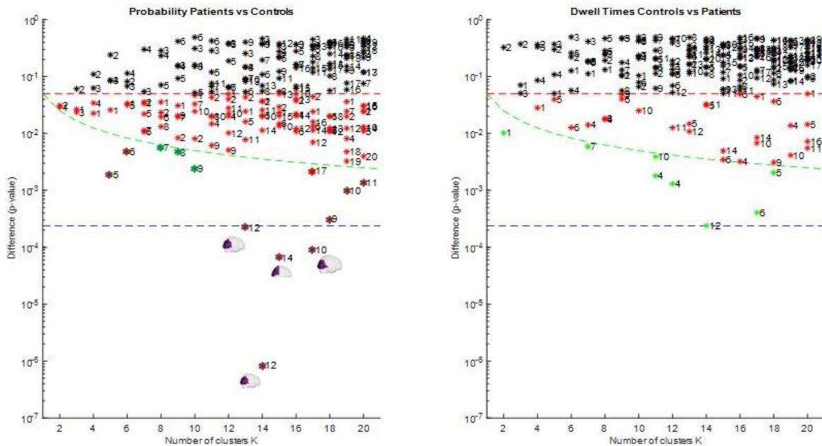
Figure 6 - Interpretation of the p values, for the probability of occurrence between states (left) and for the probability of dwell time at each state (right).
