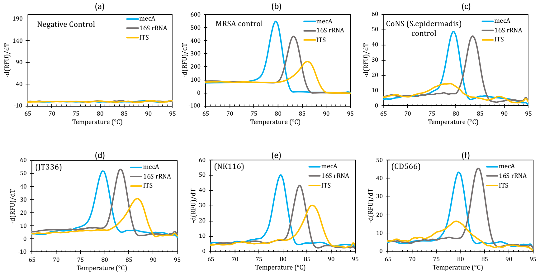
Figure 4. Melt curve analysis (MCA) for identifying CoNS contamination in the discordant samples. (a) to (c) Melt curves for three control samples and (d) to (f) three representative samples (JT336, NK116 and CD566)
