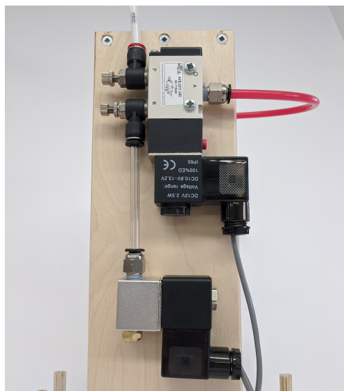
Figure 4: Close-up view of the pneumatic valves. The compressed air input is in the upper left.
