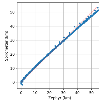
Figure 5: Calibration of the spirometer. (Left) calibration setup showing the spirometer in series with the Honeywell flow meter and a small pressure regulator to sweep the flow. The results are shown in (Right).
