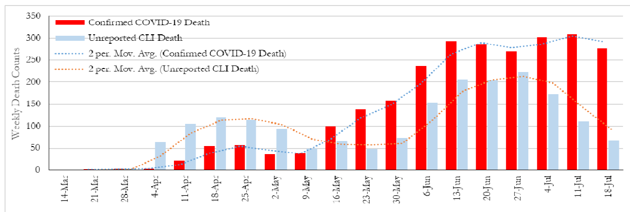
Fig. 1. Weekly confirmed COVID-19 and unreported CLI death counts, March 8–July 18, 2020, Bangladesh. The horizontal axis indicates the last date of the respective week.
