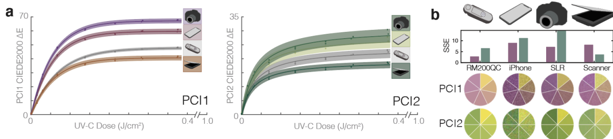
Figure 4. The potential applications for UV-C quantification from PCIs could be broadened using widely-available color measurement tools. (a) Comparison of calibration curve fits of CIEDE2000 \Delta E from an unexposed sensor vs. UV-C dose, for PCI1 and PCI2 colors quantified using the digital SLR and iPhone X in a light box, RM200QC spectrophotometer, and flatbed scanner. Dots denote individual PCI measurements, line denotes best fit, shaded region denotes 95% confidence interval on prediction of color change from observation of UV-C dose. (b) Squared sum of the residuals (SSE) for each curve fit in (a), along with color comparison wheels showing indicator color at various doses as captured by the different imaging devices. Quantification of the dose-dependent relative uncertainty for each of the 8 curve fits is presented in Supplementary Figure S11.
