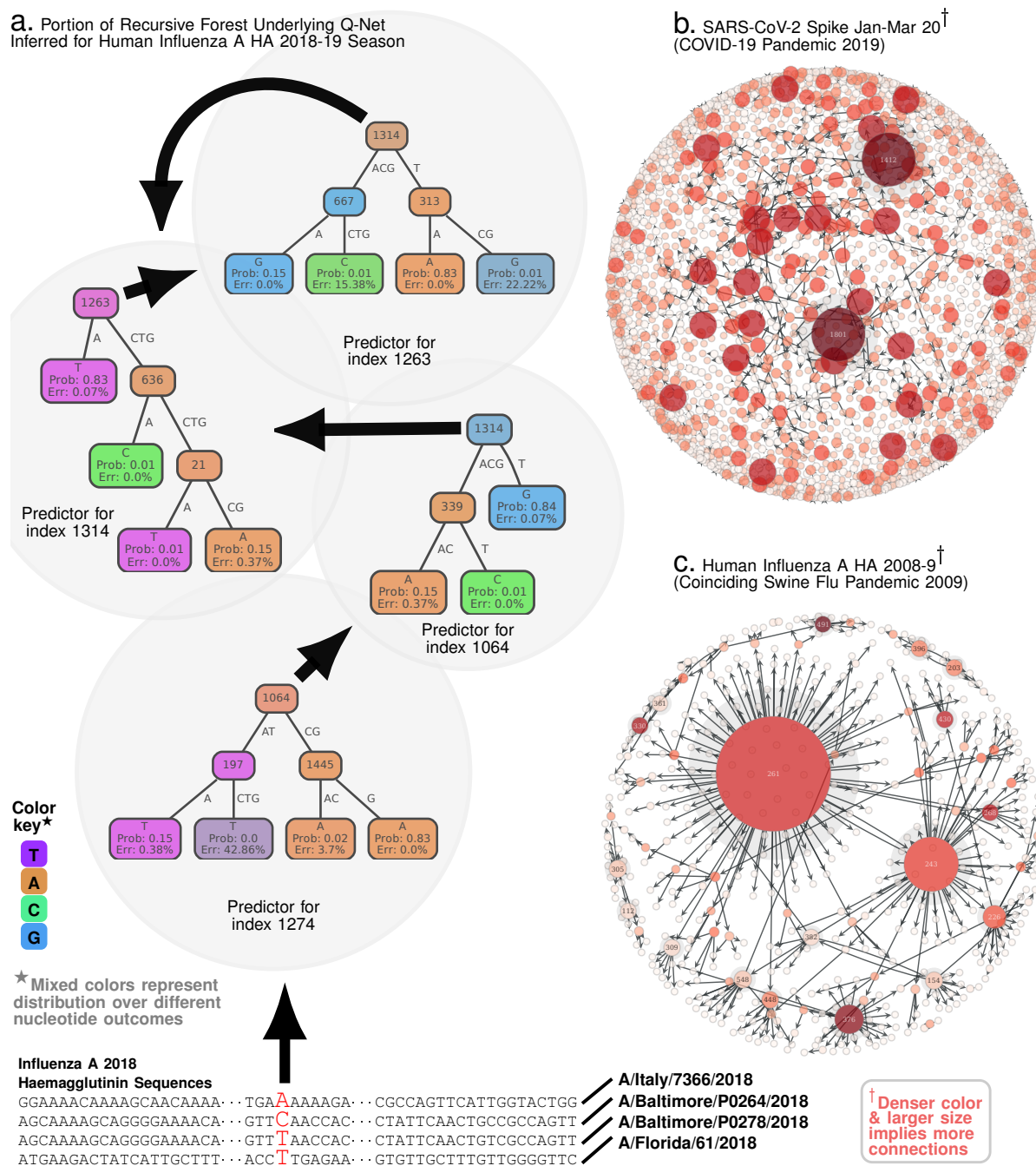
Fig. 2. Qnet Computation Scheme. Panel a. As an example, beginning with aligned sequences, we calculate a conditional inference tree for index 1274, which involves indices 1064, 1445, 197 as predictive features. These features are automatically selected by the algorithm, as being maximally predictive of the base at 1274. Then, we compute predictors for each of these predictive indices, e.g. we show the inference tree computed for index 1064, which involves index 1314 and 339 as features. Continuing, we find that the predictor for 1314 involves indices 1263, 636 and 21, and that for 1263 involves 1314, 667 and 313. Note that recursive dependencies arise automatically: the predictor for 1263 depends on 1314, and for 1314 depends on 1263. Panels b-c show Qnet dependency graphs for SARS-CoV-2 spike protein and Influenza A HA respectively, illustrating the distinct patterns of mutational constraints inferred. Both HA in Influenza A and the spike protein in SARS-CoV-2 are implicated in viral entry into host cells, and crucial for host specificity of infections. Additionally, the inferred structures underscore the significantly more complex dependencies in SARS-CoV-2 compared to Influenza A.
