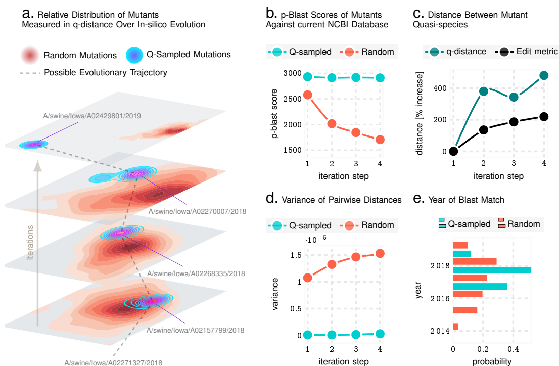
Fig. 3. Q-distance validation in silico using Influenza A sequences from NCBI database. Panel a illustrates that the Qnet induced modeling of evolutionary trajectories initiated from known haemagglutinin (HA) sequences are distinct from random paths in the strain space. In particular, random trajectories have more variance, and more importantly, diverge to different regions of the landscape compared to Qnet predictions. Panel b-e show that unconstrained Q-sampling produces sequences maintain a higher degree of similarity to known sequences, as verified by blasting against known HA sequences, have a smaller rate of growth of variance, and produce matches in closer time frames to the initial sequence. Panel c shows that this is not due to simply restricting the mutational variations, which increases rapidly in both the Qnet and the classical metric.
