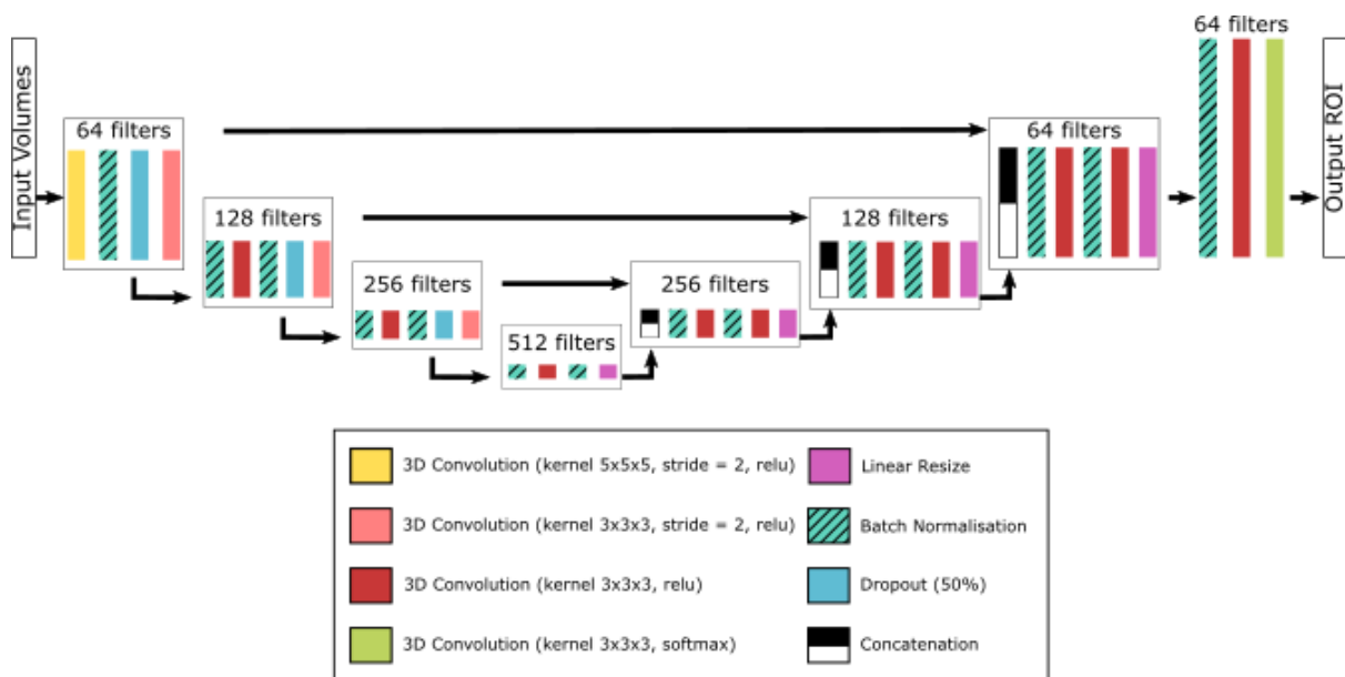
Suppl Fig 2. Neural Network Architecture.
