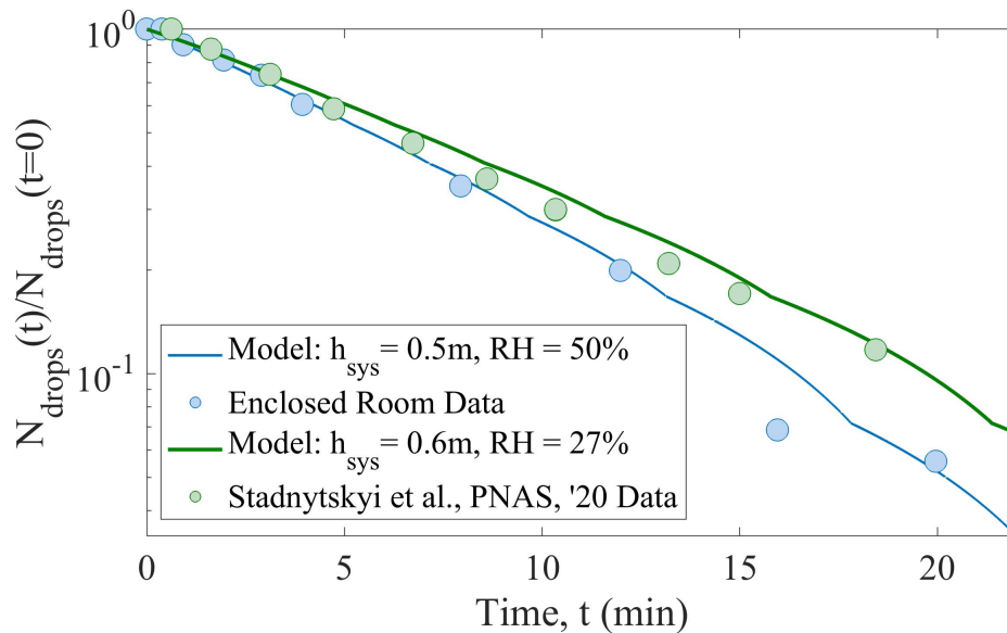
Figure 3 – Normalized number of droplets as a function of time as determined experimentally (blue circles) compared to the data of Ref. 3 (green circles). Solid lines are model fits for both sets of data, with input parameters relative humidity (RH) and sedimentation height ( h_{sys} ).
