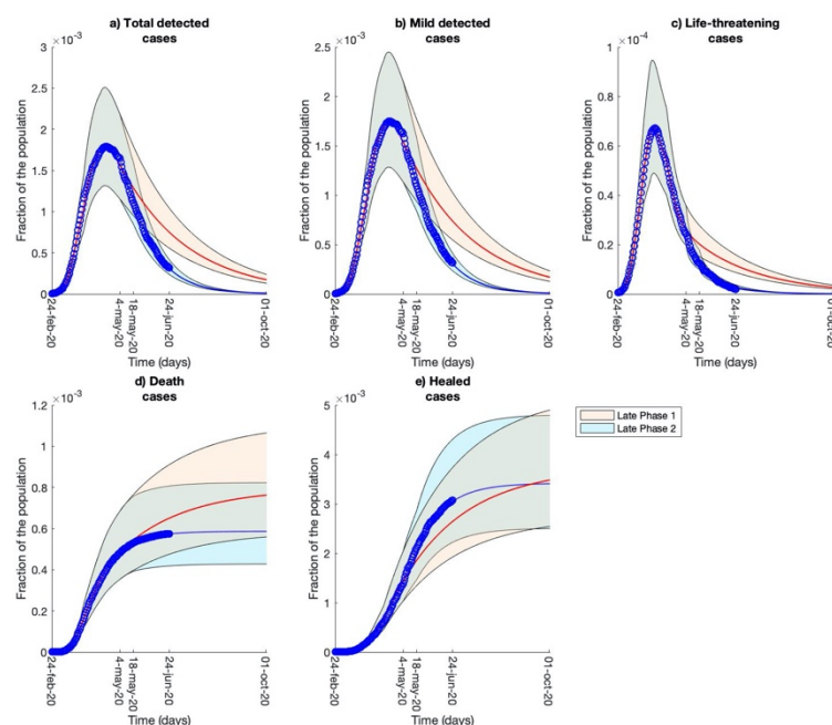
Figure 3: Comparison of model predictions. Comparison between long-term predictions based on the parameter estimates of late Phase I (from April 14th to May 4th, in red) and of late Phase II (from May 18th until June 24th, in blue). For each prediction, we reported the first, second and third quartiles. The blue dots represent the Italian data used for the calibrations.
