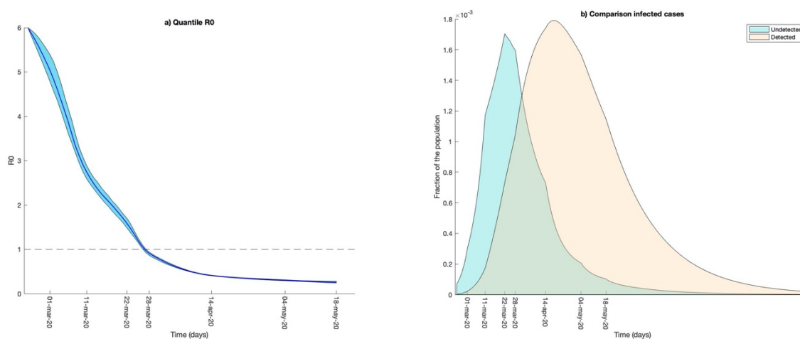
Figure 2: R0 and infected cases. From the repeated model calibrations, we computed the distribution of the model parameters and the corresponding distribution for R0 . Besides, since the model accounts also for undetected individuals, we can compare the distribution of detected and undetected cases along time. a) R0 distribution. The light blue shade represents the values between the first and the third quartiles computed with the estimate distribution of model parameters obtained from the repeated model calibrations. The dark blue line represents the second quartile of the distribution. b) Comparison between undetected cases (variables I and A in the model) and detected cases (variables D , R and T in the model).
