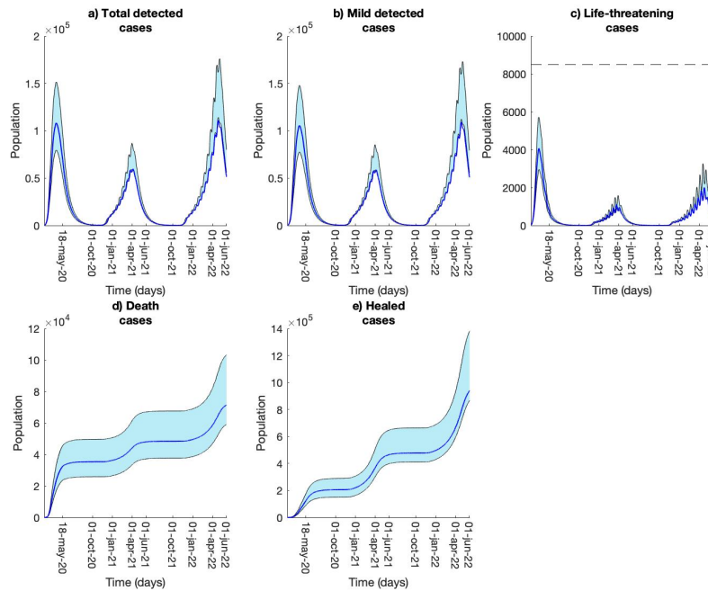
Figure 4: Long-term prediction with seasonal component and intermittent lockdown. Long-term model predictions computed by including a seasonal component to the contagion parameters and an intermittent lockdown policy. The lockdown alternates between 6 “open days” (no lockdown) and 8 “close days” (complete lockdown) when the epidemic situation worsens. The first peak refers to the first epidemic wave that we experienced in the period February-June 2020. The second and the third peaks are predictions for 2021 and 2022, respectively. The plots represent the first, second and third quartiles; the time length of the simulations goes from February 2020 until June 2022. The dashed horizontal line in panel c) is the maximum ICU capacity for Italy, reported as 8940 beds 31,32 .
