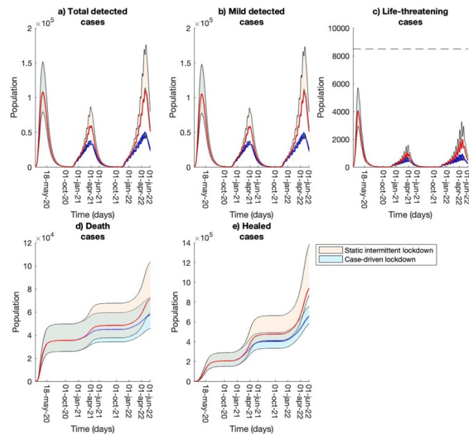
Extended Figure 4: Long-term prediction with different intermittent lockdown policies. Comparison between long-term model predictions computed with different intermittent lockdown policies. The red curves represent an intermittent lockdown with a fixed number of 6 “open days” alternated with 8 “close days” during the months from October to June (scenario presented in Figure 4). The blue curves describe an intermittent lockdown that is driven by the number of daily infected cases. Specifically, the “close days” start when there are more than 500 daily new infections for at least 3 days. The “open days” start when the daily infections go below 250 cases for at least one week. During the period October - June, the lockdown alternates a mean of 8 “open days” with 12 “close days”. In both the two scenarios we included the seasonal component for the contagion parameters.
