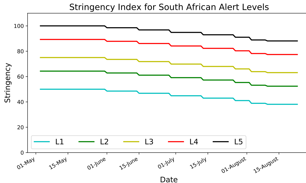
Figure 1: Time Varying Stringency Index for each South African Alert Levels 1-5.
