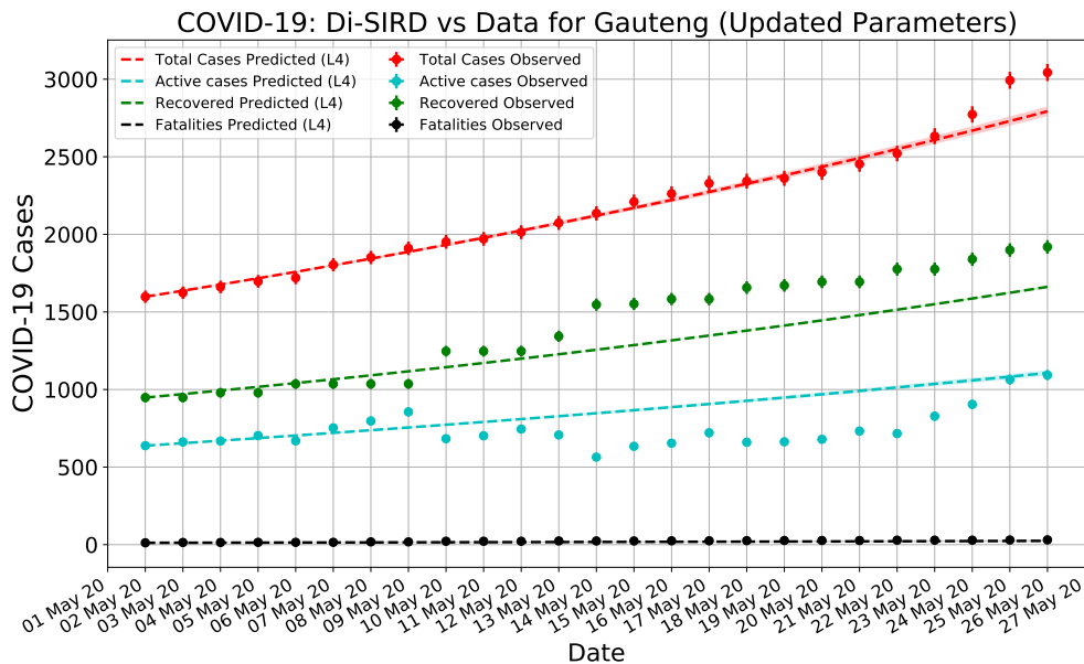
Figure 5: Gauteng province predictions versus data with re-calibrated parameters using Level 4 stringency (see text).
