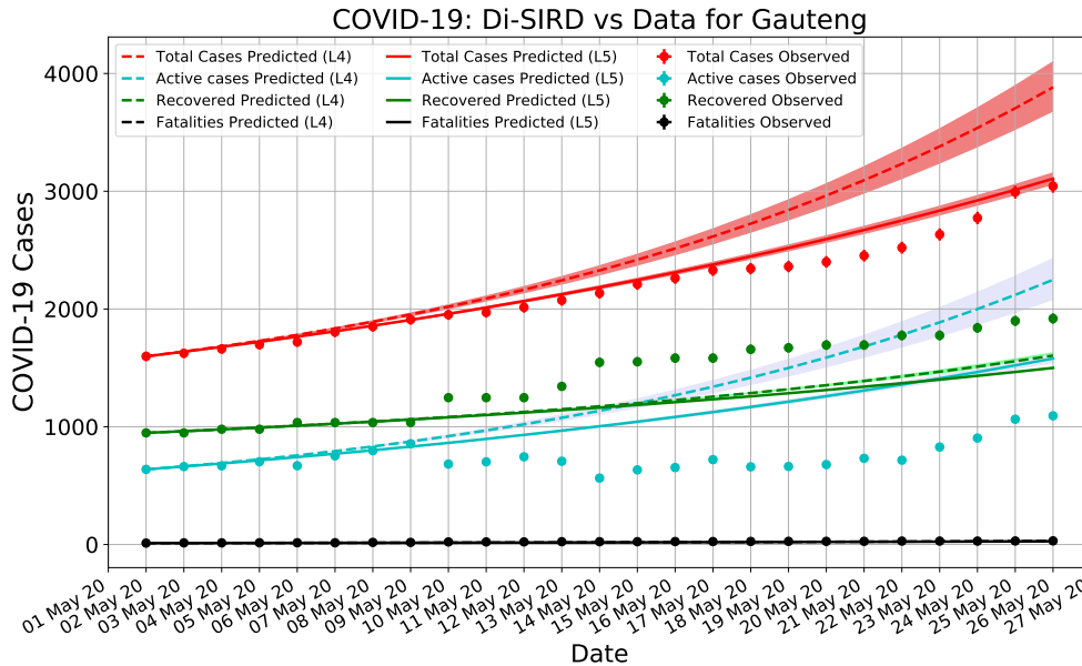
Figure 4: Gauteng province predictions versus data for alert Levels 4 and 5 using the parameters obtained during lockdown (see text).
