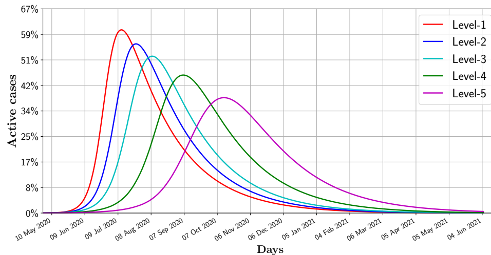
Figure 2: Predictions for South Africa in terms of the differential distribution of active cases for the different alert levels (see text).
