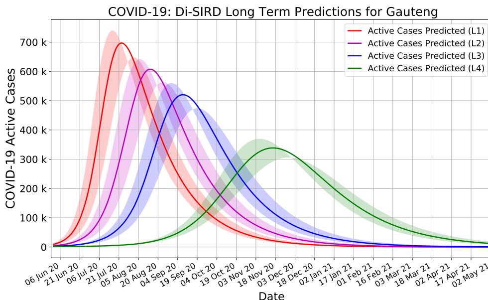
Figure C.8: Long term re-calibrated predicted number of active cases in Gauteng Province
