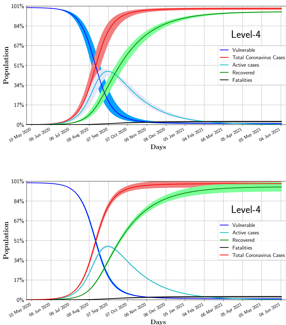
Figure C.7: Uncertainties of the model for Level 4 restrictions. The upper and lower graphs correspond to uncertainties in \alpha_s and \gamma_0 , respectively (see text).
