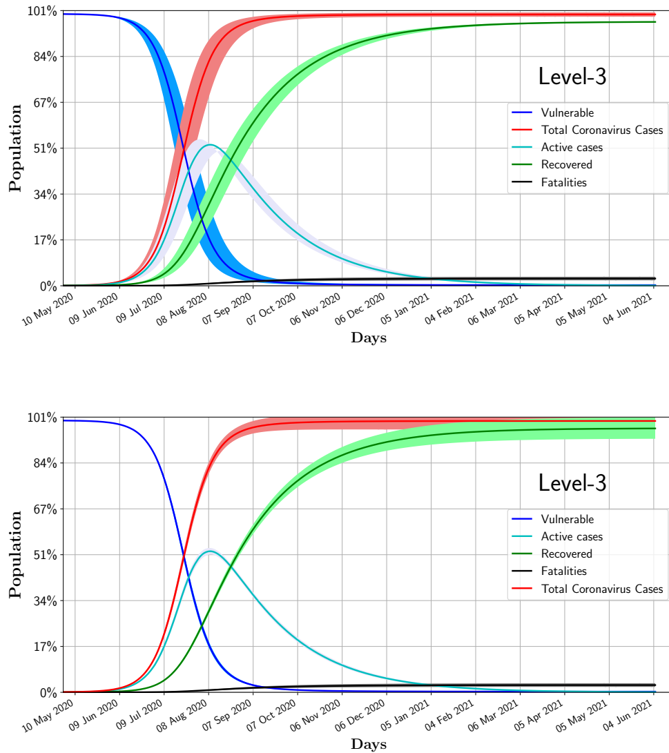
Figure 3: Uncertainties of the model for Level 3 restrictions. The upper and lower graphs correspond to uncertainties in \alpha_s , \beta_0 and \gamma_0 , respectively (see text).
