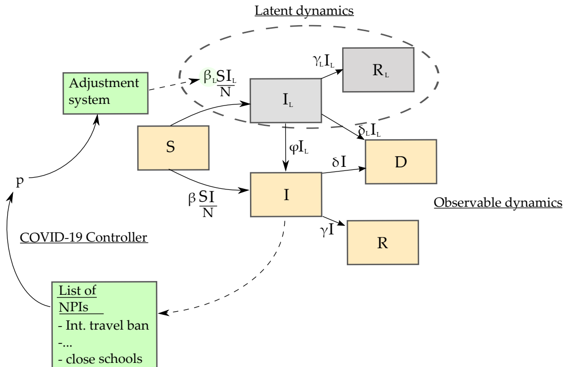
Figure 6: Latent SIRD model with NPI controller of the latent transmission parameter \beta_L . Extended from Choma et al. 2
