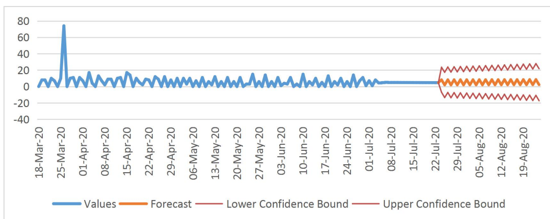
(b) ARIMA-311, death cases-West Bengal
