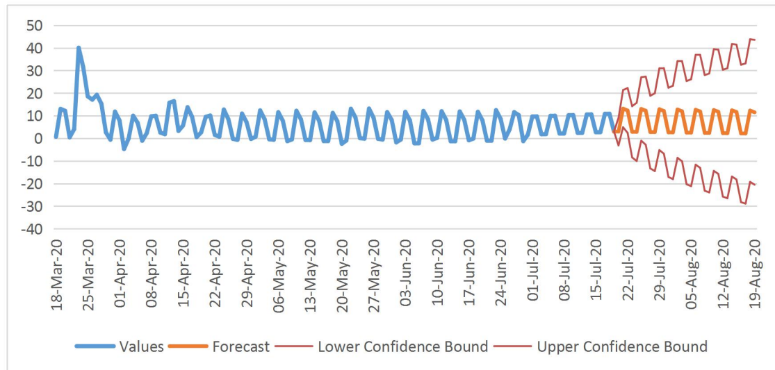
(a) West Bengal-death cases- Holt-Winters (0.3,0.3)
