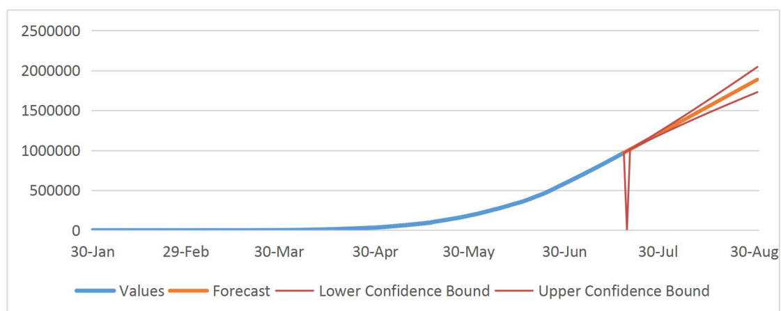
Figure 3: Forecasting for the confirmed cases (ARIMA-411): India
