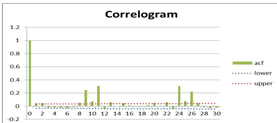
(c) ACF for death cases
