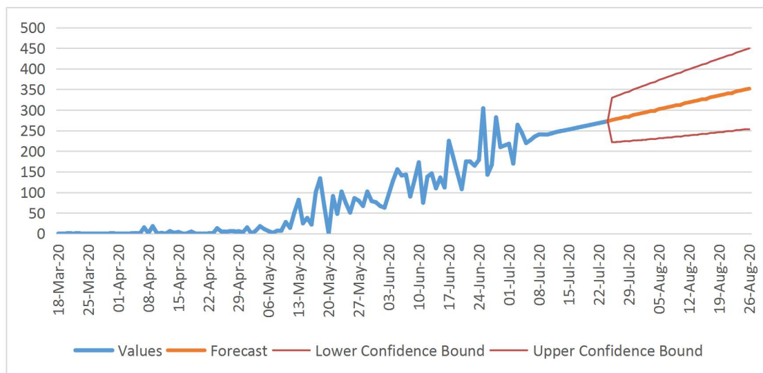
Fig 11: ARIMA and Holt-Winters forecasting for the confirmed cases and death cases For Andhra Pradesh
