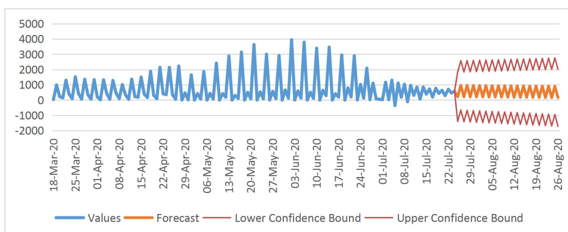
A. ARIMA-411, confirm cases-Delhi
