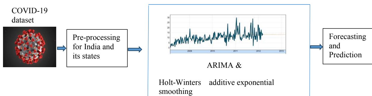
Figure 1: Proposed time series forecasting method
