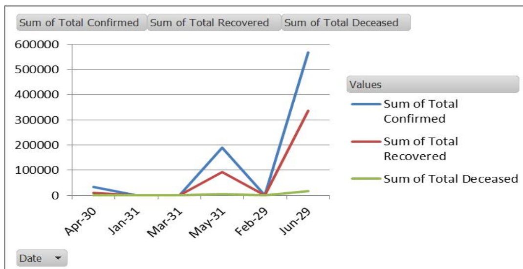
Fig 5: India statistics for COVID-19 spreading
