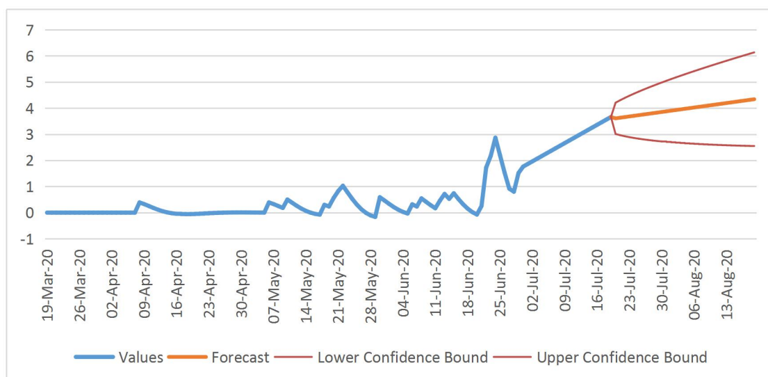
Fig 12: ARIMA and Holt-Winters forecasting for the confirmed cases and death cases for Odisha
