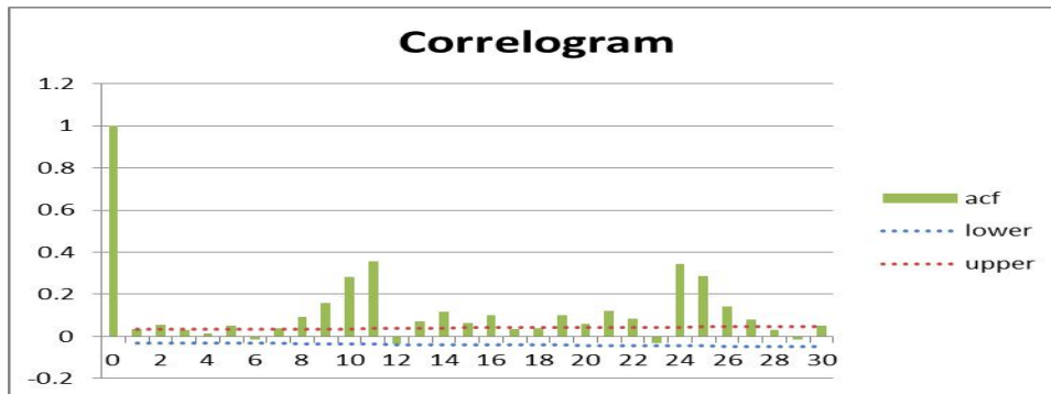
(a) ACF for confirm cases
