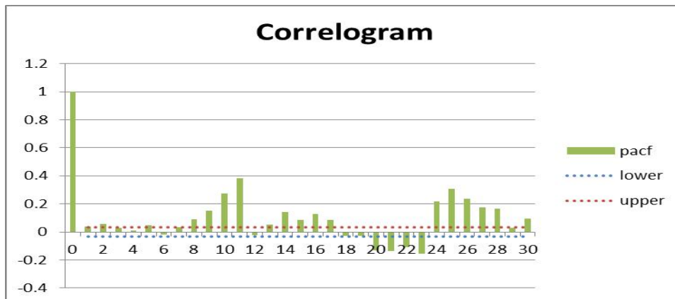
(b) PACF for Confirm cases
