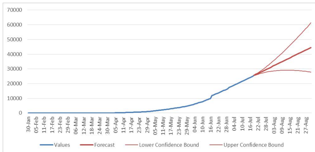
Figure 4: Forecasting for the death cases (ARIMA-311): India
