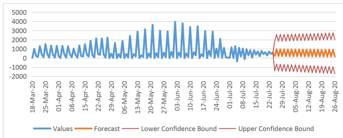
A. ARIMA-411, confirm cases-Delhi
