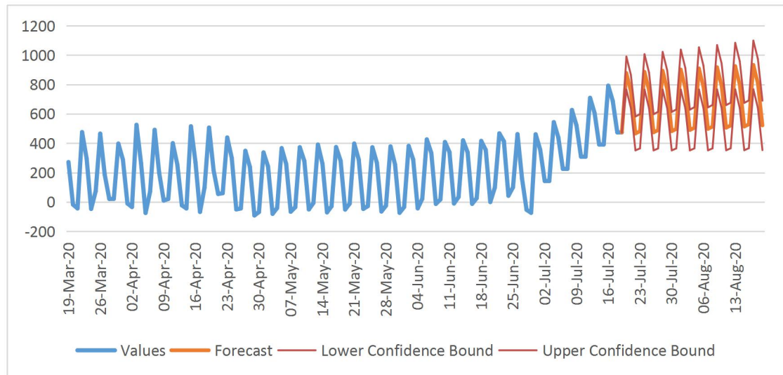
(b) West Bengal-confirm cases- Holt-Winters (0.3,0.3)
