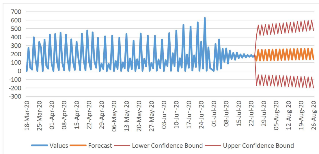
(a) ARIMA-411, confirm cases-West Bengal
