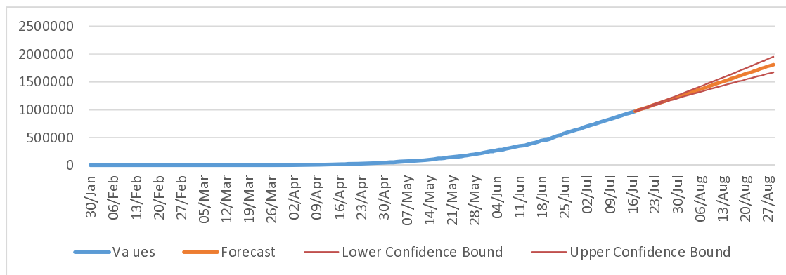
Figure 6: Holt-Winters forecasting for cumulative confirm cases in India
