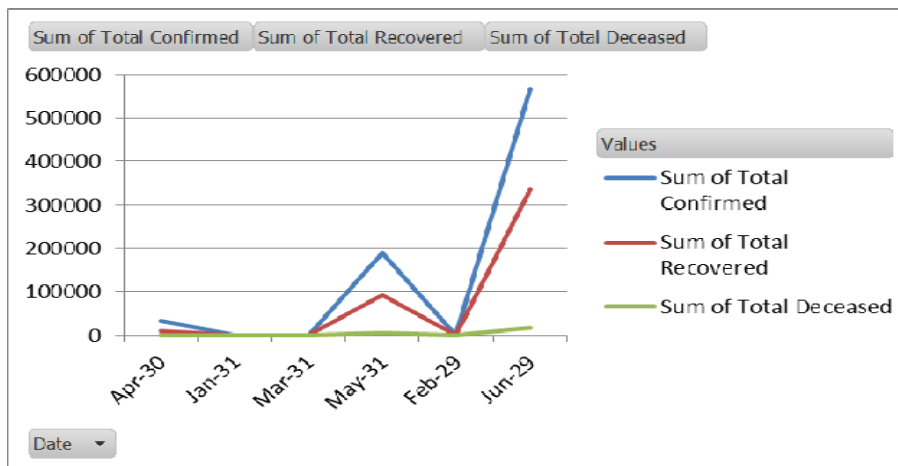
Fig 5: India statistics for COVID-19 spreading
