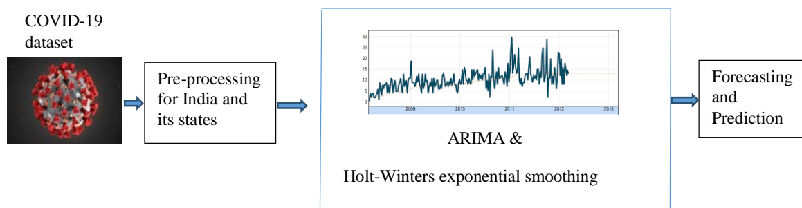
Figure 1: Proposed time series forecasting method
