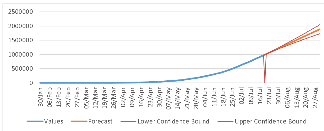
Figure 3: Forecasting for the confirmed cases (ARIMA-411): India
