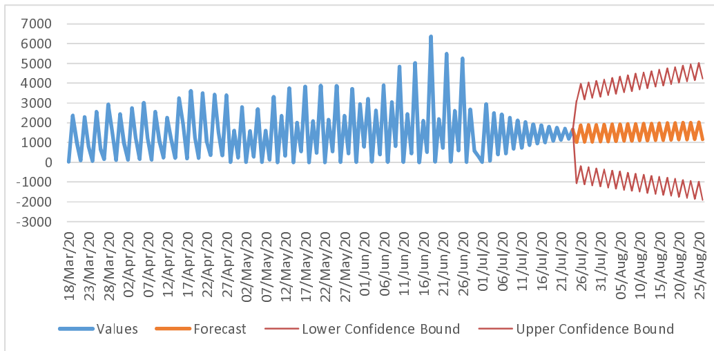
Fig 9: ARIMA and Holt-Winters forecasting for the confirmed cases and death cases For Delhi
