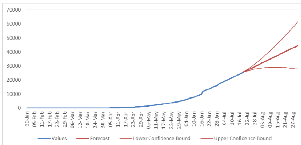
Figure 4: Forecasting for the death cases (ARIMA-311): India
