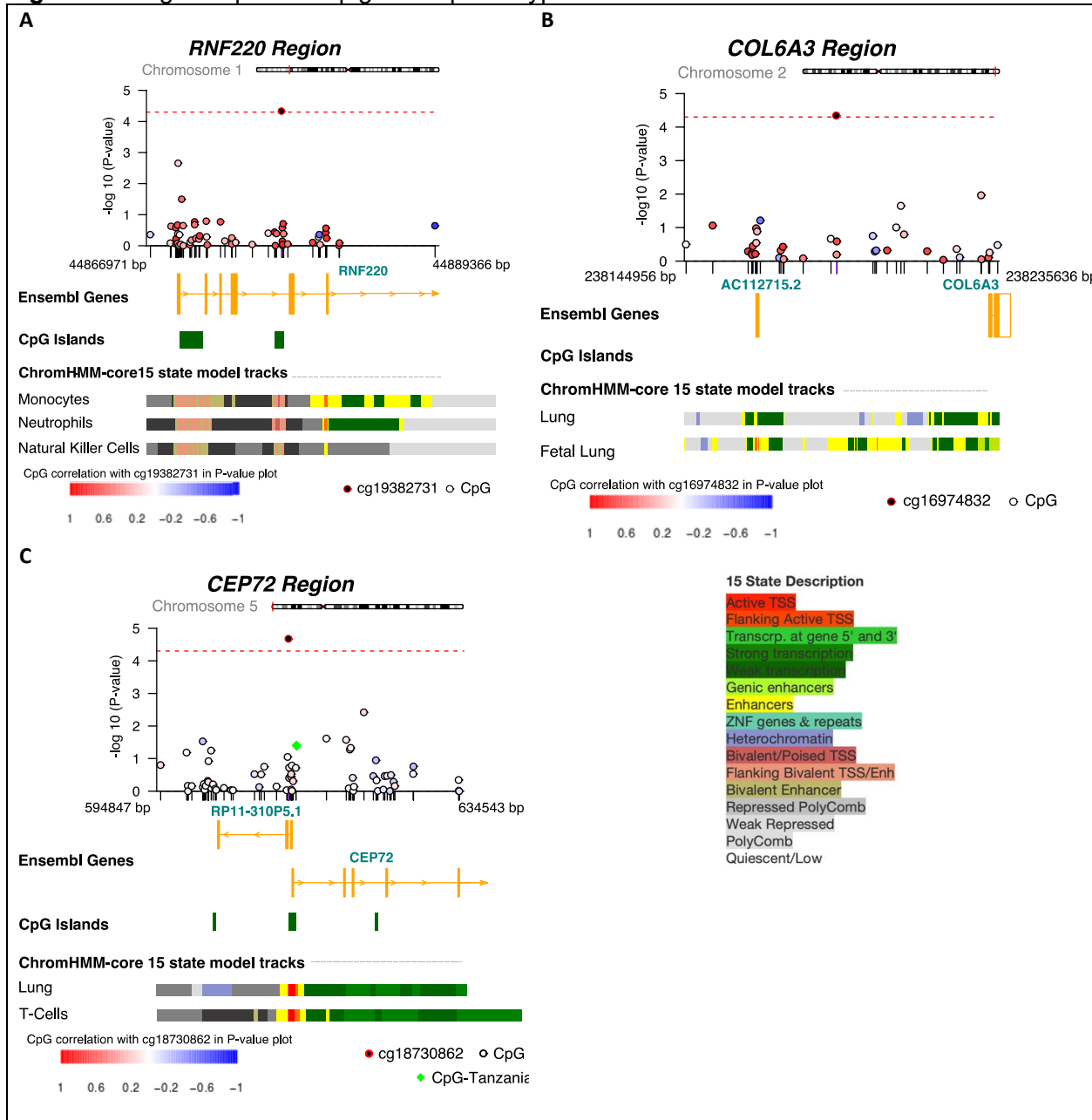
Figure 2. Regional plots of epigenetic-phenotype association results
