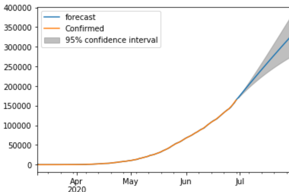
Figure 2: Prediction for a period from 10 March 2020 to 01 August 2020 confirmed cases in Maharashtra
