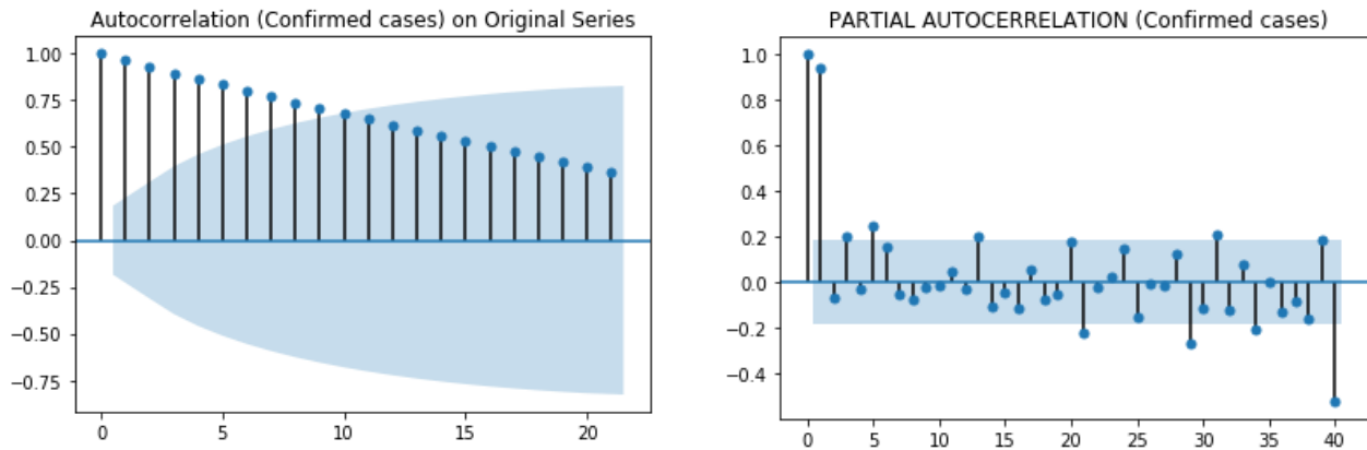
Figure 1: Autocorrelation and PACF plot for confirmed cases in Maharashtra
