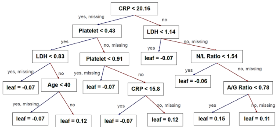
Figure 2: Decision rules using the key features under the Day-1 simplified model and their thresholds.
