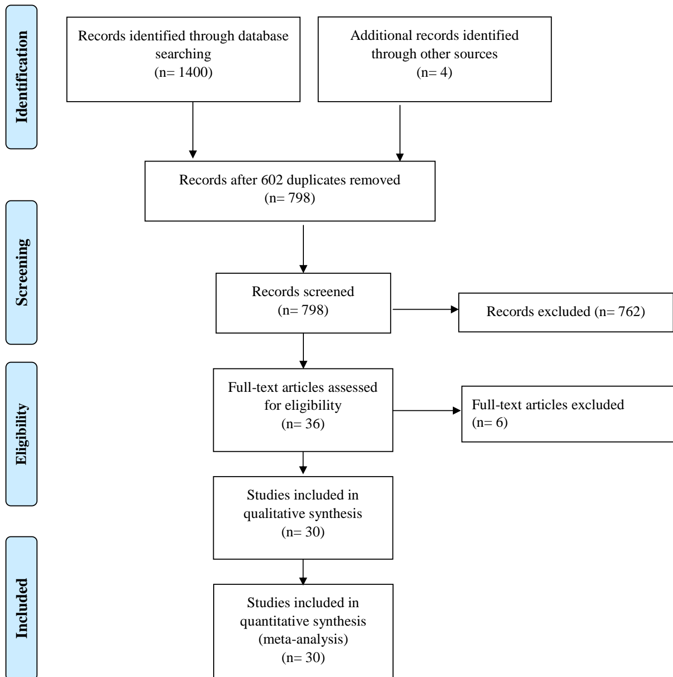
Figure S1: Flowchart of study selection process in accordance with PRISMA guidelines.
