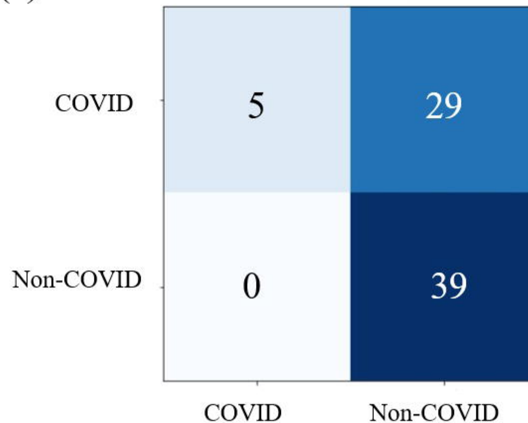
ResNet-50
