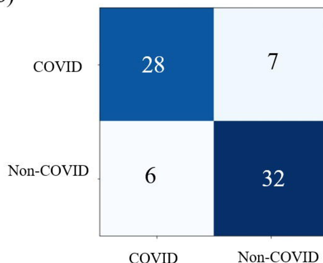
CTnet-10
