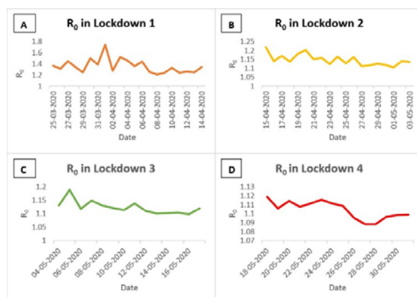
Fig 2 Plot showing the Scenarios of Different lockdown with R_0 values of COVID-19 in India
