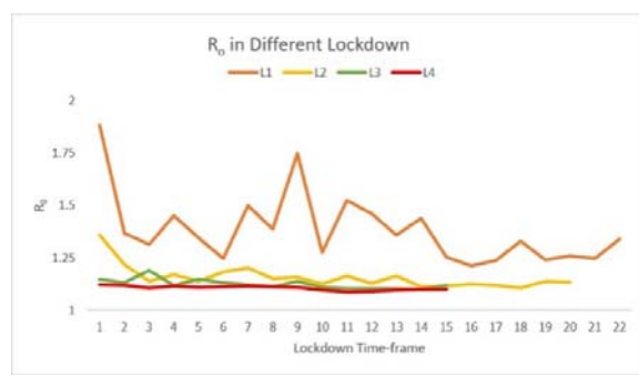
Fig 3 A comprehensive analysis chart define the transmission of corona virus reproduction rate ( R_0 ) in varies lockdown time frame in India
