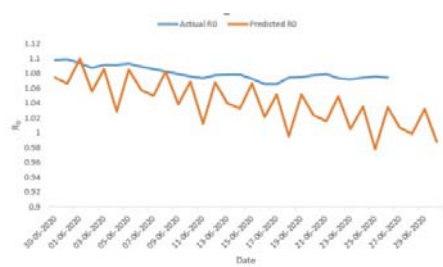
Fig 5 Comparison between actual (without lockdown) and predicted R0 values (if lockdown sustain in month of June) for month of June.
