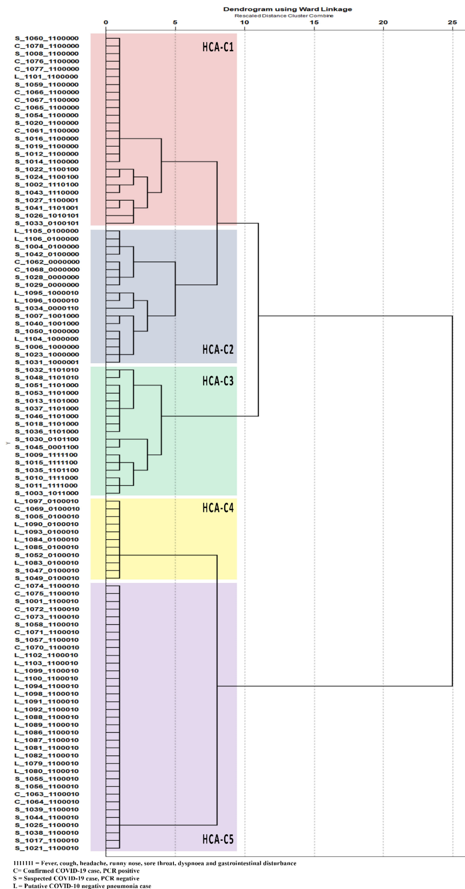
Figure 1. Dendrogram of symptoms cluster for confirmed and suspected COVID-19 cases, and non-COVID-19 pneumonia patients
