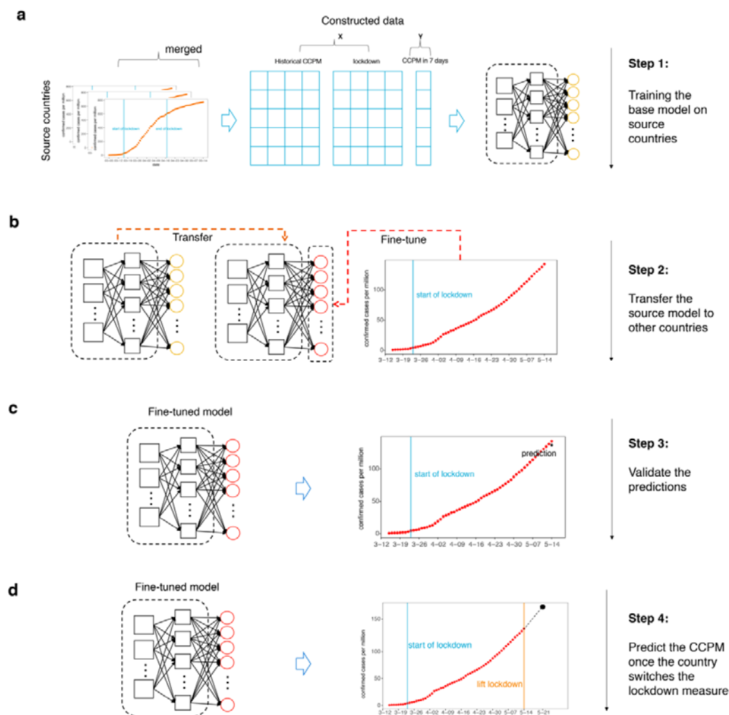
Figure 2. Schematic representation of the computational steps of ALeRT-COVID. a , The source model was trained on the source set constructed from the source countries. b , The source model was fine-tuned on each training set constructed from the corresponding target country. c , The fine-tuned model (target model) was validated on each test set constructed from the corresponding target country. d , The target model was utilized to predict the future CCPM (Confirmed Cases per Million) for the countries once the governments switch the lockdown measures.
