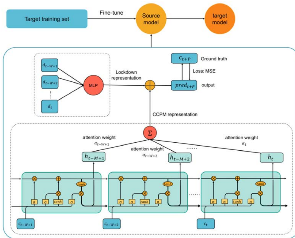
Figure 6. Architecture of ALeRT-COVID.
