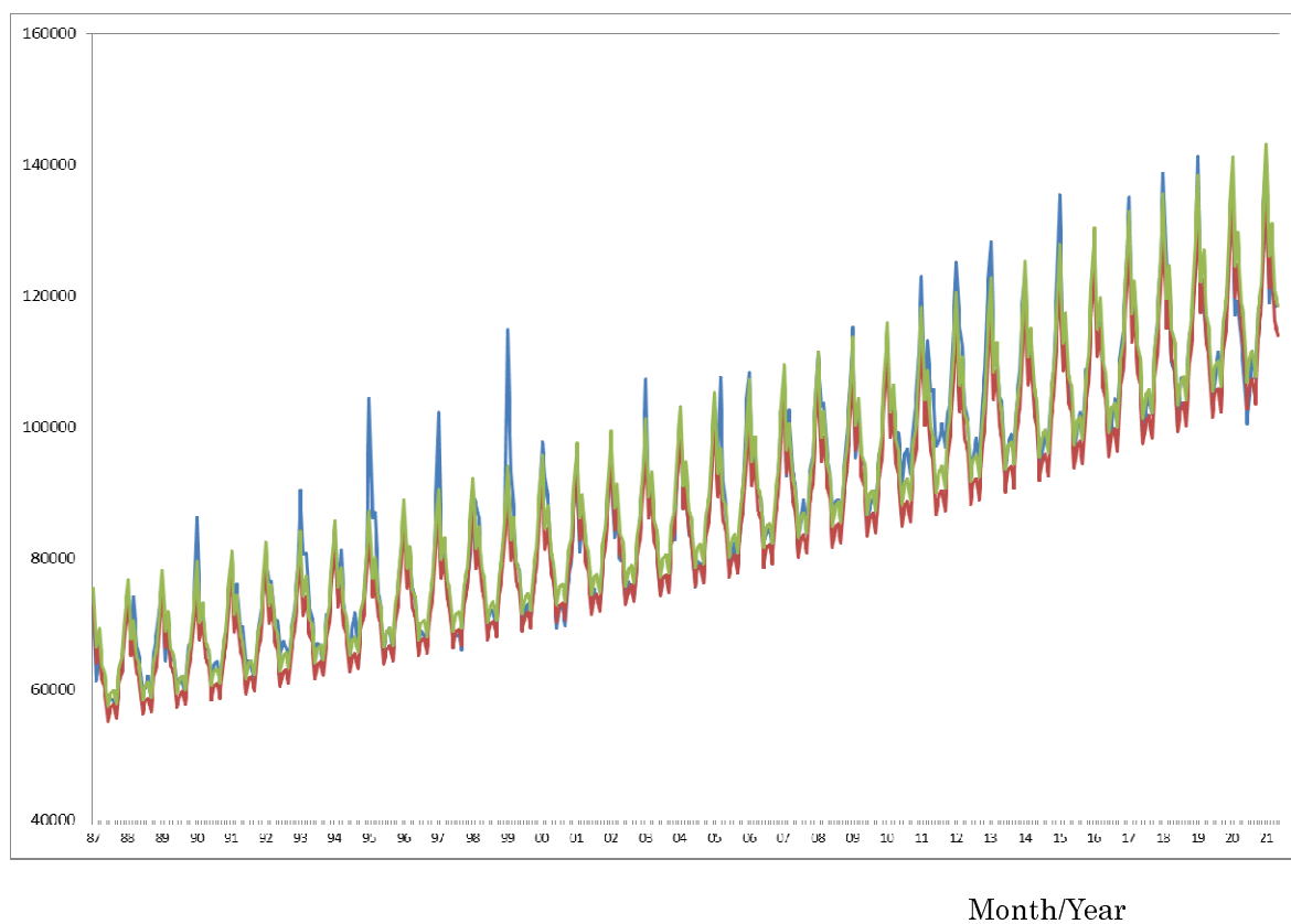
Figure 1: Observations of the estimated baseline and threshold since 1987 until May 2021 in Japan (persons)
