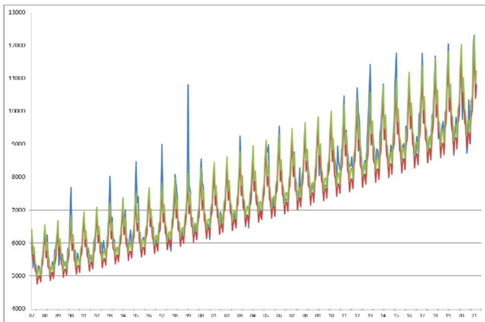
Figure 3: Observations of the estimated baseline and threshold since 1987 until February 2021 in Tokyo (persons)
