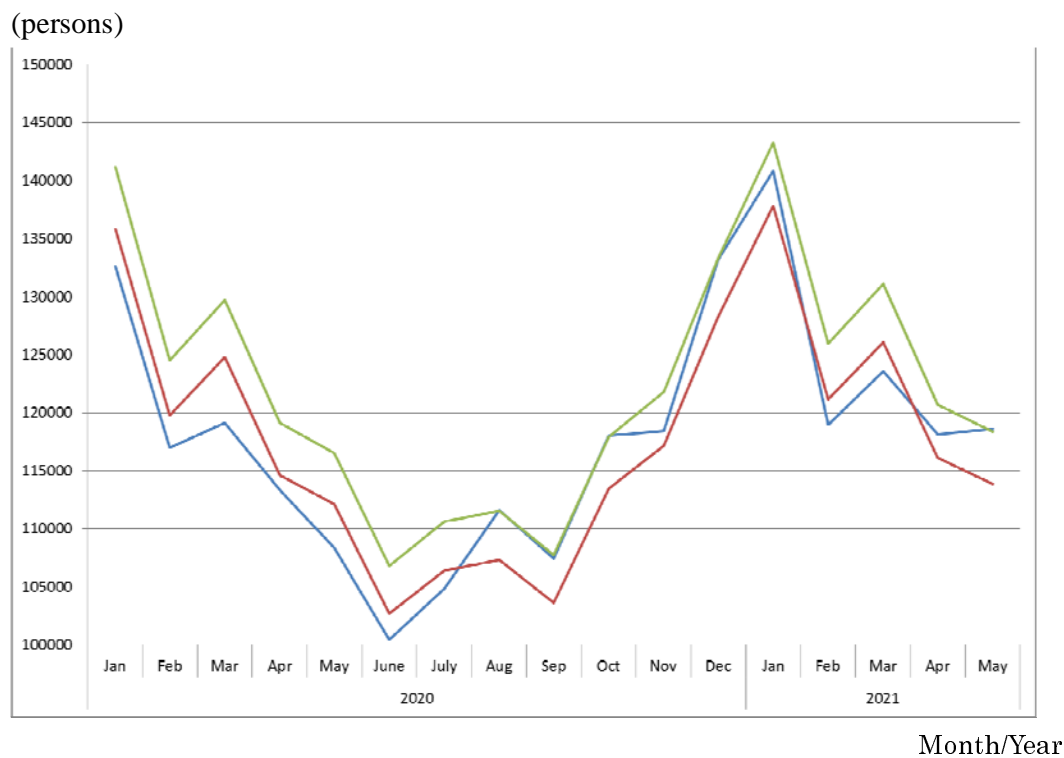
Figure 2: Observation of the estimated baseline and threshold since January 2020 in Japan
