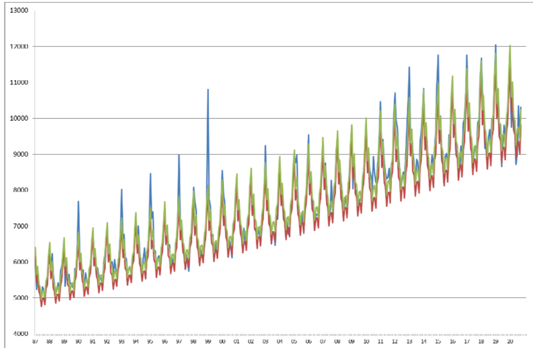
Figure 3: Observations of the estimated baseline and threshold since 1987 until October 2020 in Tokyo (persons)
