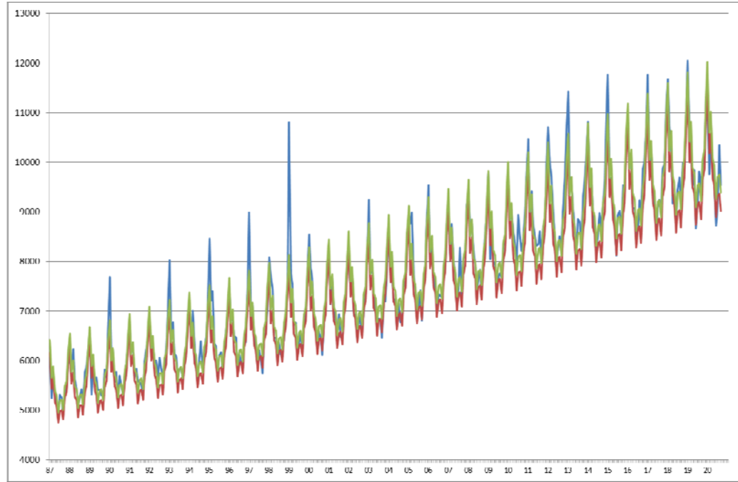
Figure 3: Observations of the estimated baseline and threshold since 1987 until September 2020 in Tokyo (persons)
