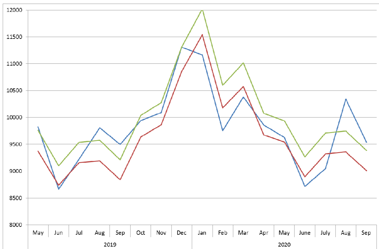
Figure 4: Observation of the estimated baseline and threshold since May 2019 until September 2020 in Tokyo (persons)
