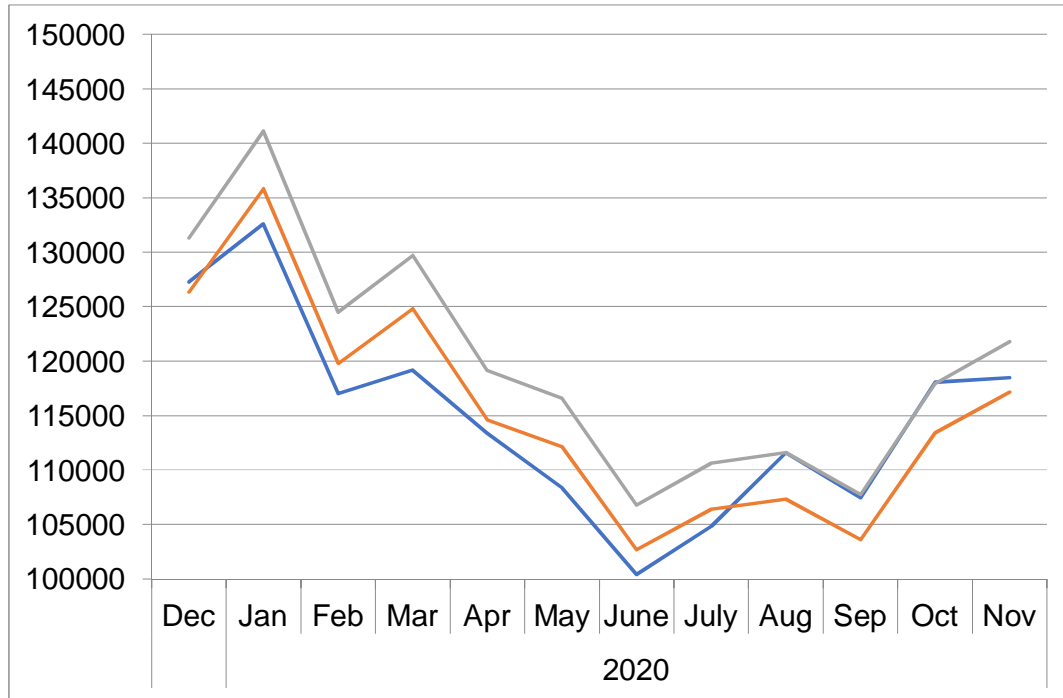
Figure 2: Observation of the estimated baseline and threshold since December 2019 in Japan (persons)
