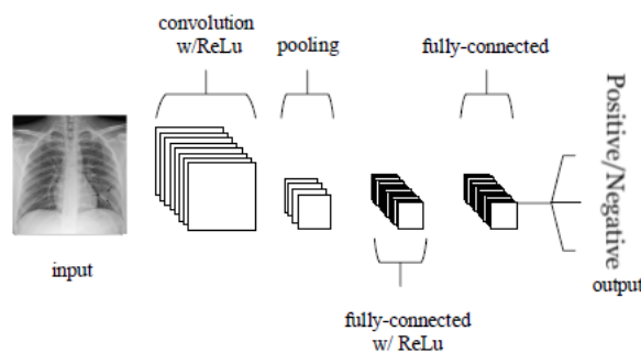
Fig. 4. CNN Architecture.
