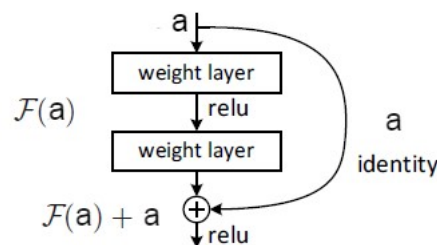
Fig. 5. ResNet block diagram [5].
