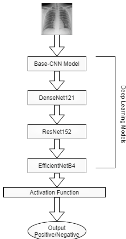
Fig. 2. Block diagram of our methodology.
