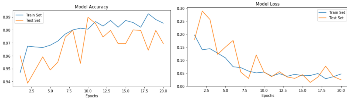
Fig. 7. From left side, (a) Model accuracy of EfficientNetB4 model and (b) Model loss of EfficientNetB4 model.
