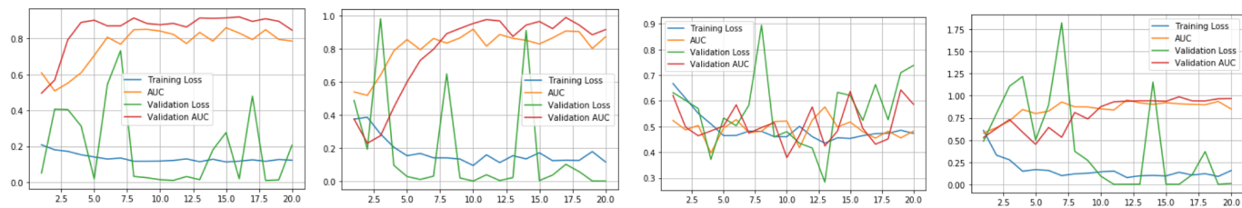
Fig. 6. From left side, (a) Base CNN performance graph; (b) ResNet152 performance graph; (c) DenseNet121 performance graph and (d) EfficientNetB4 performance graph.
