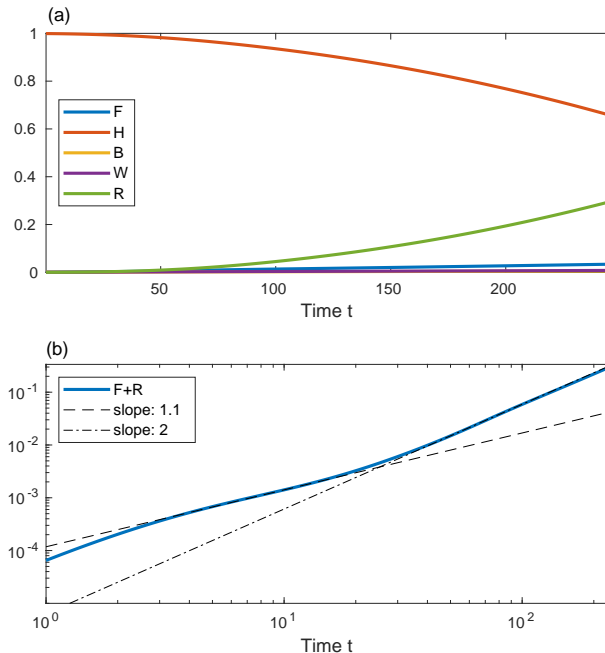
FIG. 5. Global population curves it vs time corresponding to the circular infection centers in Fig. 4. Compare to the cases of uniform (Fig. 1) or random (Figs. 2-3) distributions of 'b'. Dashed and dash-dotted curves are linear fits at t = 10 and t = 83 , respectively.
