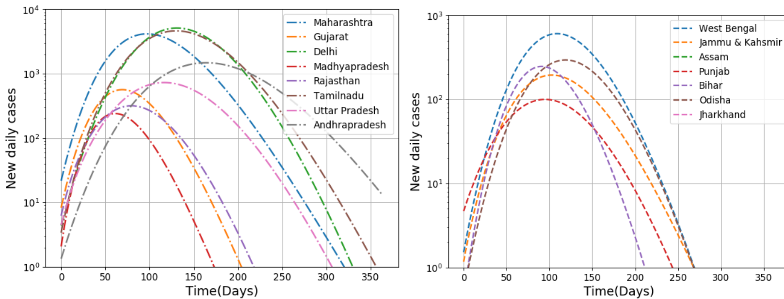
Fig. 6 (a) and (b): Predicted new daily infected cases in various selected states of India by SIRD model
