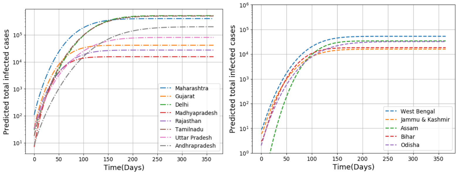
Fig. 4 (a) and (b): Predicted total infected cases in various selected states of India by SIRD model
