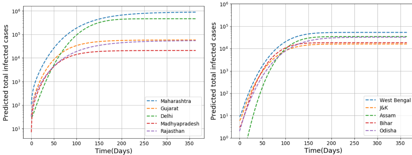
Fig. 3 (a) and (b): Predicted total infected cases in various selected states of India by SEIRD model
