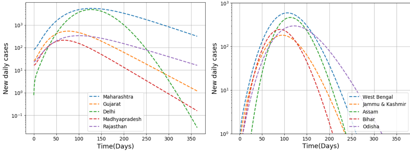
Fig. 5 (a) and (b): Predicted new daily infected cases in various selected states of India by SEIRD model
