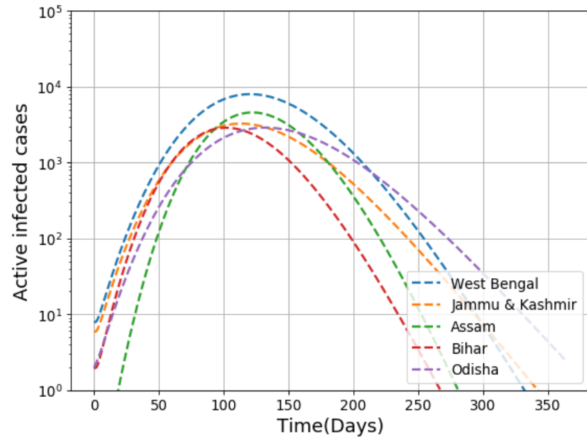
Fig 7 (a) and (b): Predicted active infected cases in various selected states of India by SEIRD model
