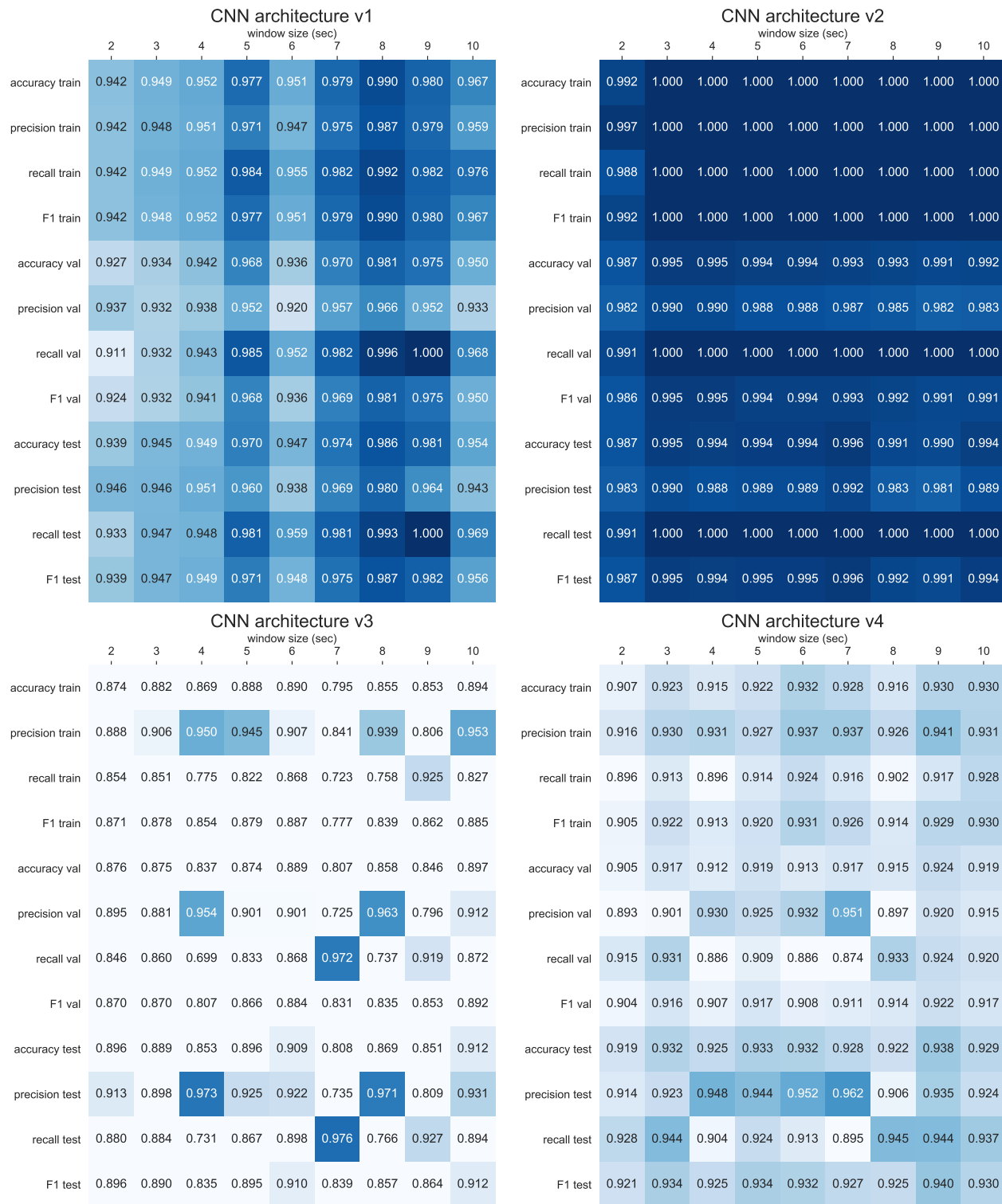
Figure 3. Accuracy, precision, recall, and F1 performance metrics for training data (60%), validation data (20%), and test data (20%) for the four architectures evaluated. All CNN models were trained for a total of 250 epochs with early stopping enabled, a patience of 25 epochs, and restoring of the best weights when the validation loss was the lowest.
