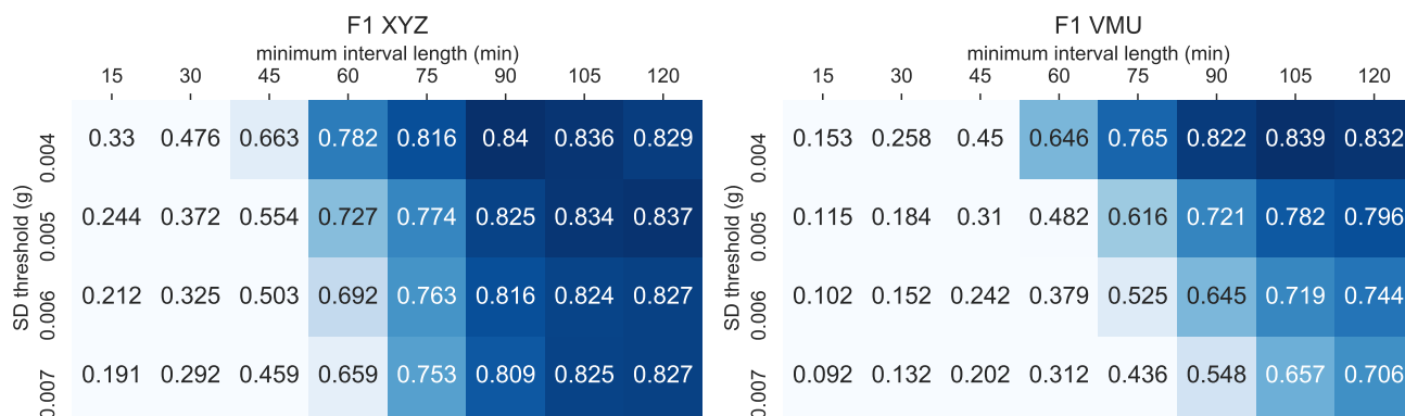
Figure 4. The F1 classification performance of the XYZ baseline algorithm (left), and the VMU baseline algorithm (right). Note that a SD threshold of 0.003 g performed poorly as it is below the accelerometer noise level and is therefore not shown. See Supplementary Fig. S4 and S5 for accuracy, precision, and recall scores.
