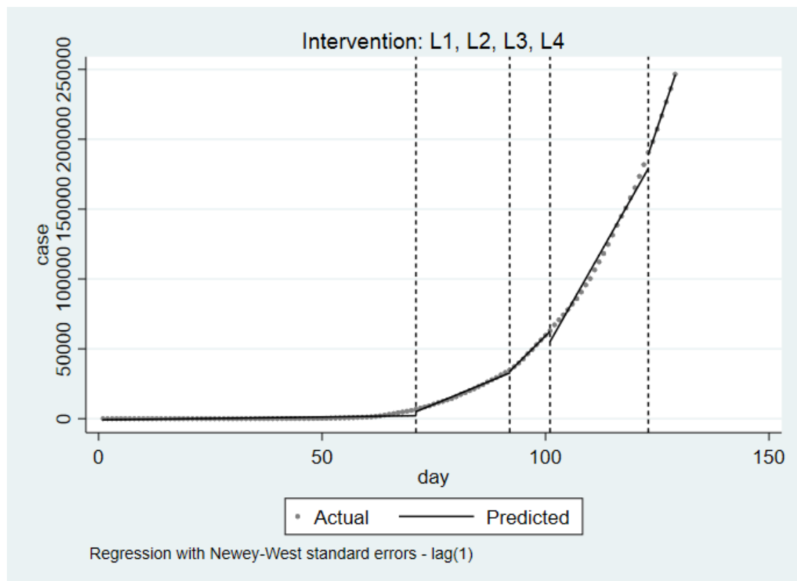
Figure 1: Impact of lockdown on COVID-cases using Interrupted Time Series model
