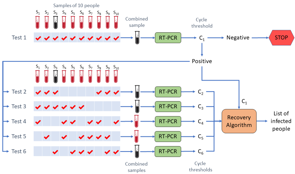
Fig. 2. Schematic of 2-STAP-I for pool size = 10.
