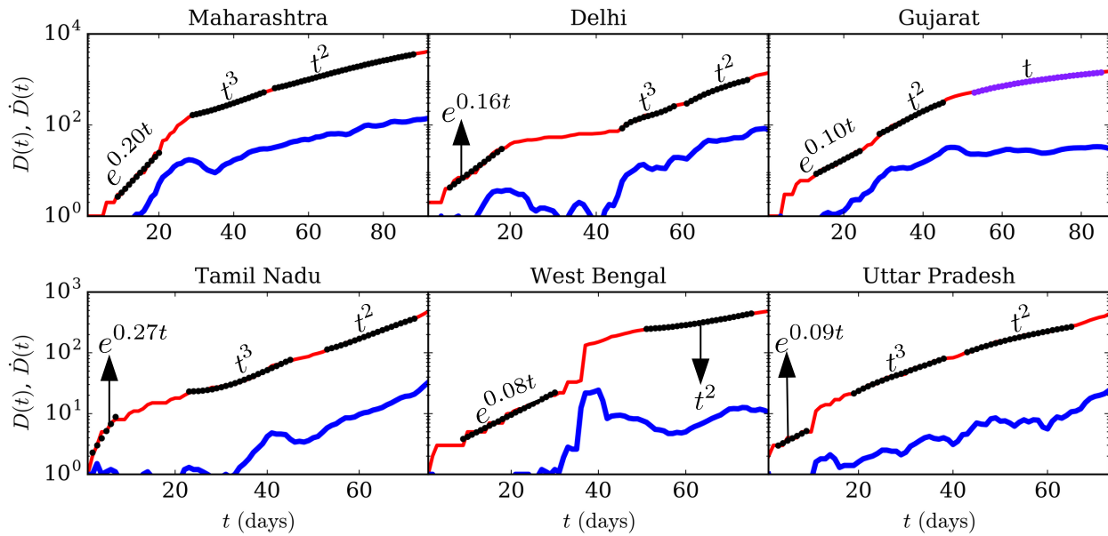
Fig. 2 (color online) The semi-log plots of total death cases ( D(t) ) vs. time ( t ) (red thin curves) and \dot{D}(t) vs. t (blue thick curves) for six states of India. The dotted curves represent the best-fit curves (see Table 2).
