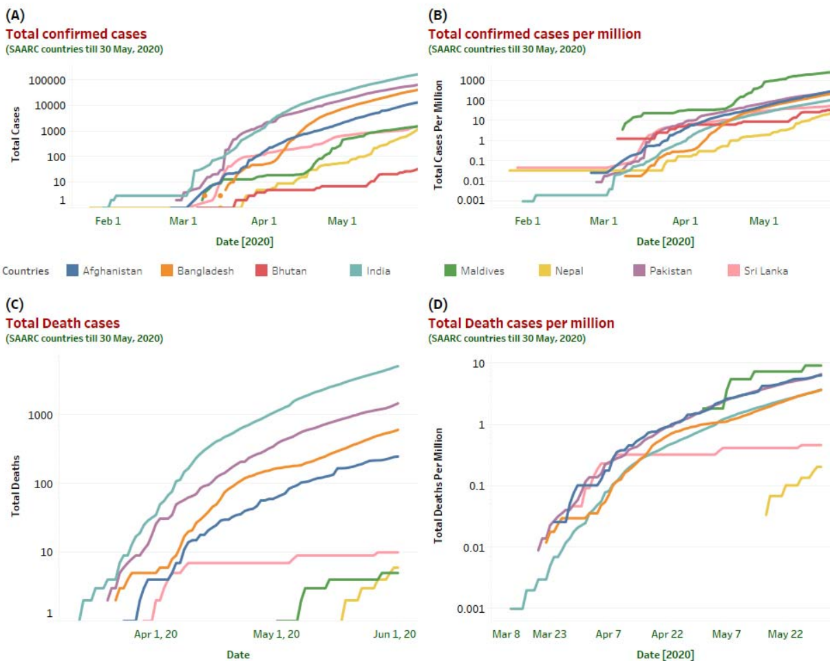
Figure 2: This graphical representation provides a comprehensive overview of the total number of confirmed and death cases in SAARC regions. Country-wise COVID-19 confirmed and death cases along with the number of cases per million illustrated in 2(A), 2(B), 2(C), and 2(D) till May 30, 2020. Based on the illustration on 2(A) and 2(C), India has confirmed the highest number of infected cases (173763) along with the most number of death cases (5164) in the region.
