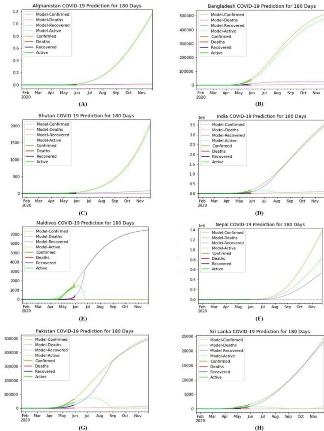
Figure 5: Long term prediction model for the next 180 days using M-SIR approach. This prediction provides a depiction of all SAARC countries evaluation of COVID-19 till Mid November. All the countries prediction curve are denoted here from (A-H) respectively.
