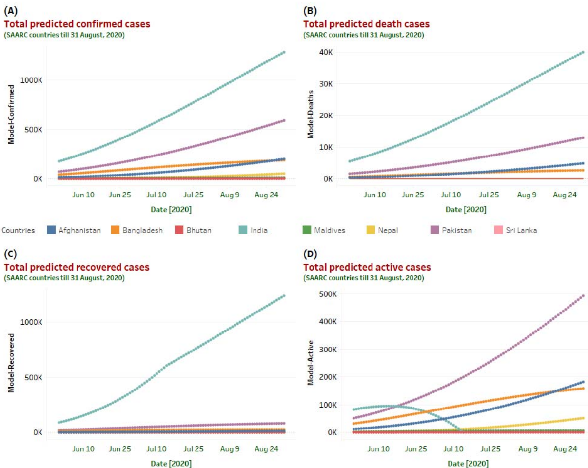
Figure 4: Based on the M-SIR prediction model, prediction statistics for the upcoming 90 days for all the countries in the SAARC regions has depicted here. Different predicted case scenarios (confirmed, death, recovered, and active) till August 31, 2020, helps to understand the epidemiological nature of COVID-19 in the south Asian region. The predicted model indicates that in the next 90 days prediction curve will increase sharply for India (in terms of confirmed and death cases). Moreover, India will also show a substantial increase in its recovery rate. However, the number of active cases will increase in Pakistan till August 31, 2020.
