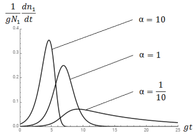
Fig. 2: Dependence of the daily number of cases on time at different values of \alpha = g_1/g_2
