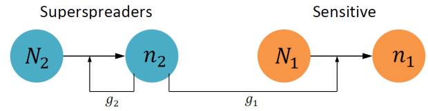
Fig. 1: Scheme of the two-component epidemic model
