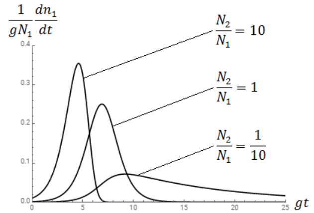
Fig. 3: Dependence of the daily number of cases on time at different values of \alpha = N_2/N_1
