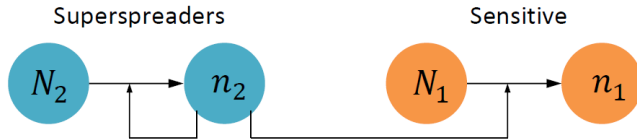
Fig. 2: Scheme of the two-component epidemic model
