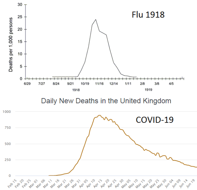
Fig. 4: Course of two epidemics in the UK: flu (1918) and COVID-19 (2020)
