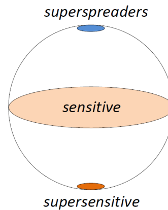
Fig. 1: Two groups of infected ( superspreaders and supersensitive ) as two opposite poles of the immune reaction
