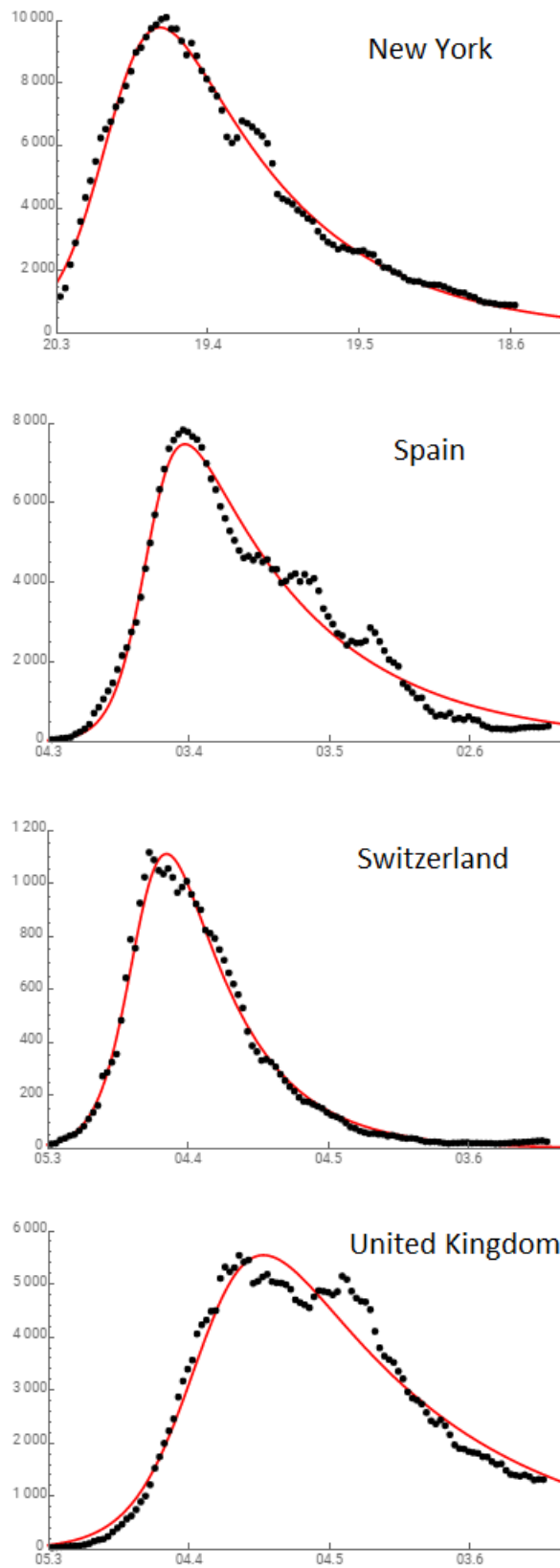
Fig. 5: Comparison of course of COVID-19 epidemic in 12 countries and territories (points) with two-component model (red line)
