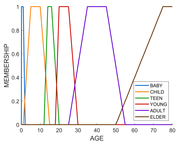
Figure 2. Piecewise linear functions representing age group membership.
