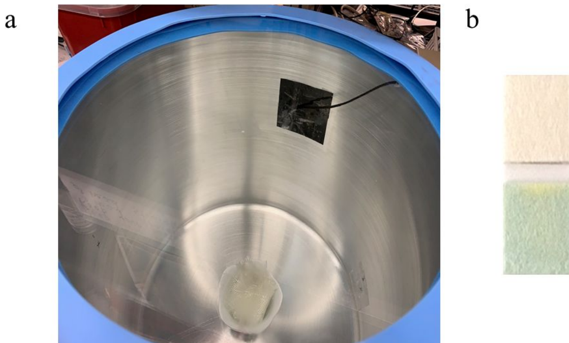
Fig. 1. a. System designed for measurement of H_2O_2 concentration inside the chamber. b. Color of the hydrogen peroxide test strip corresponding to the unexposed reference sample (top) and the exposed post-treatment sample with H_2O_2 3% weight fraction (bottom).
