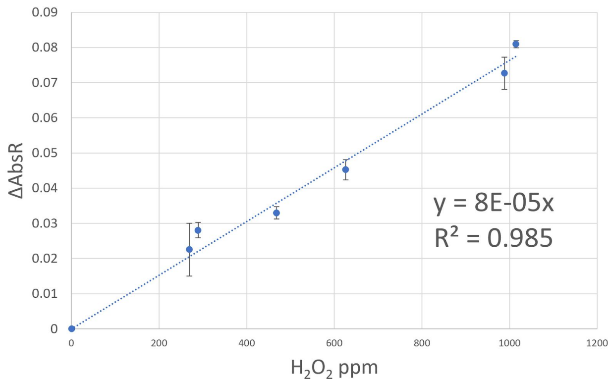
Fig. 2. Calibration curve for H_2O_2 solutions 0-5%. Error bars represent the standard deviation of the red light component absorbance.
